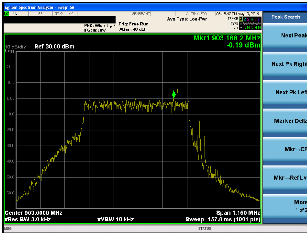
Power spectral density plot on 903.0MHz
