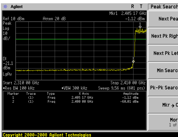
\pi/4 -DQPSK: Band Edge-Low Channel (Hopping Mode)
