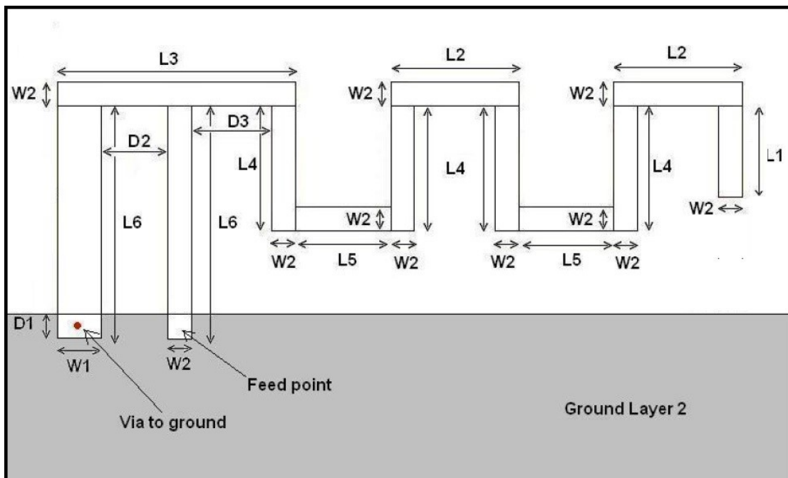
Picture: Antenna Dimensions
