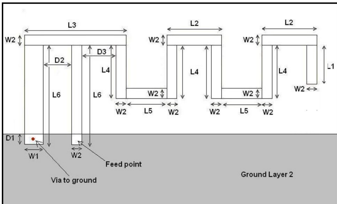
Picture: Antenna Dimensions
