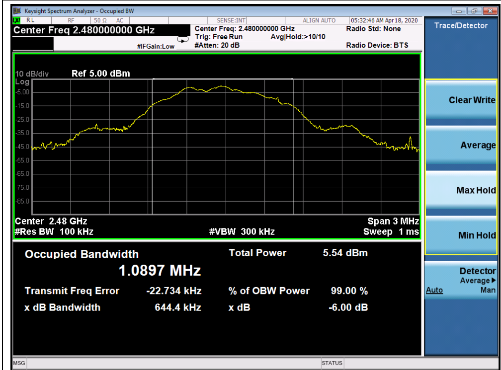
BLE-2480MHz
