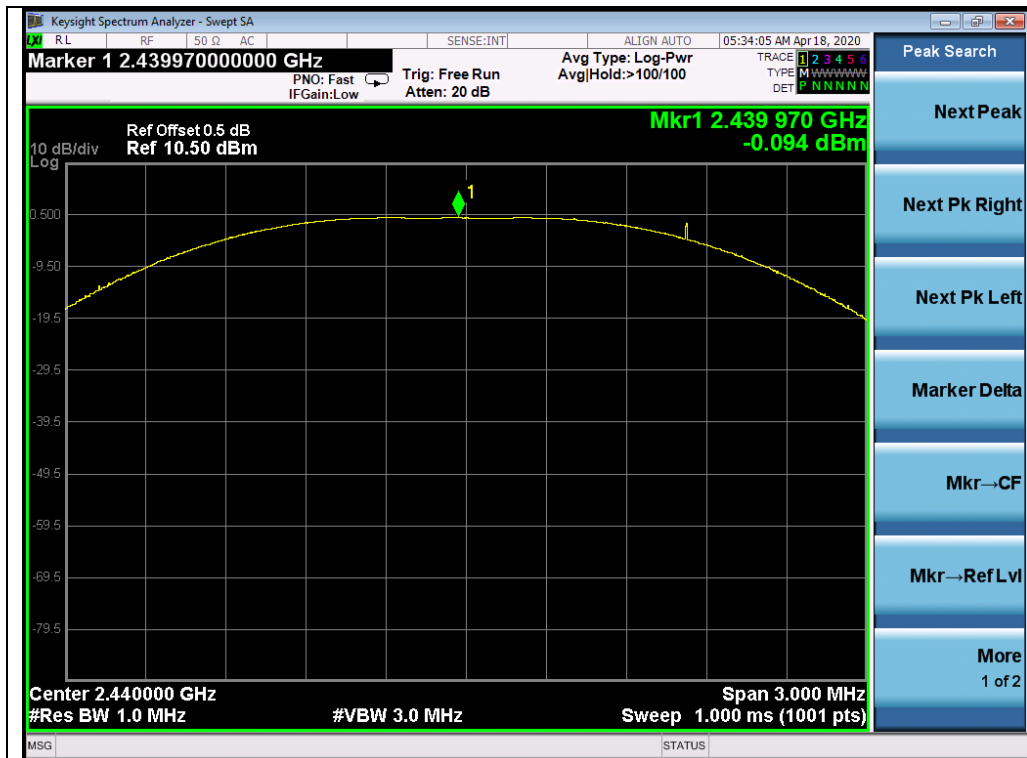
BLE-2440MHz
