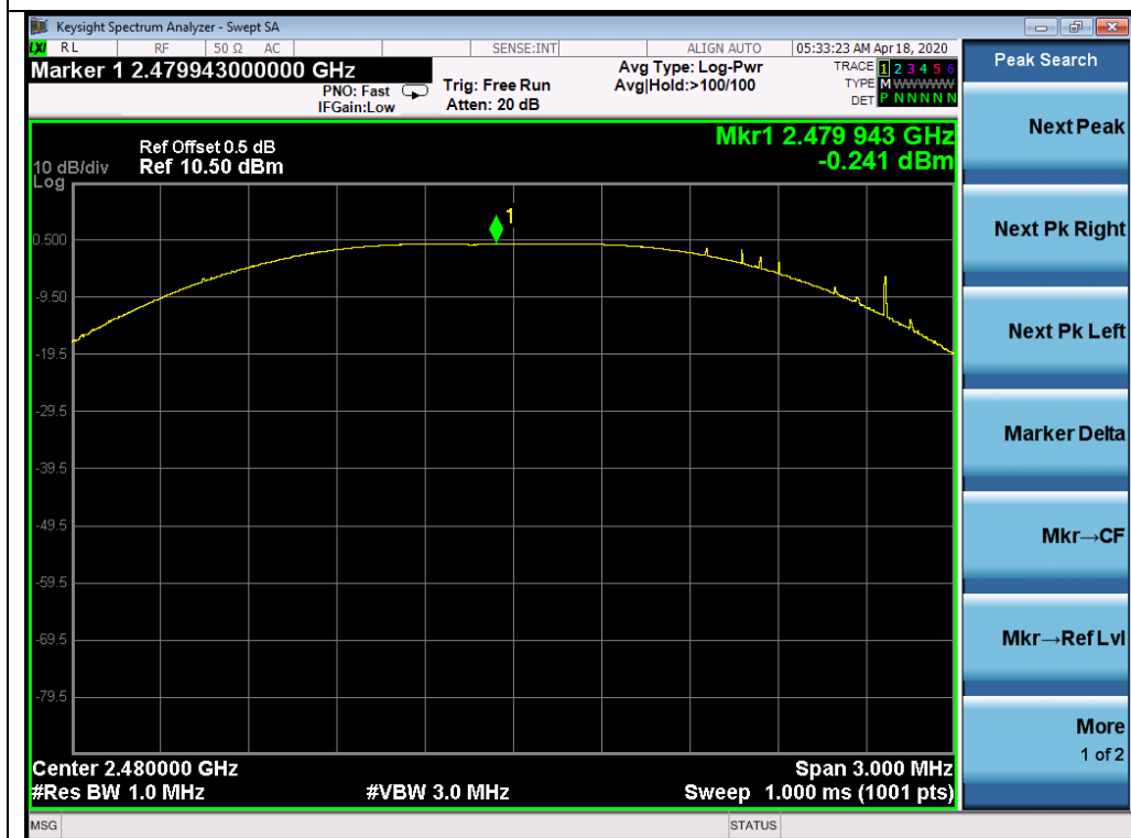
BLE-2480MHz
