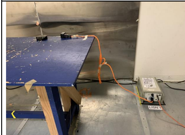
Conducted Emission Test Front View
