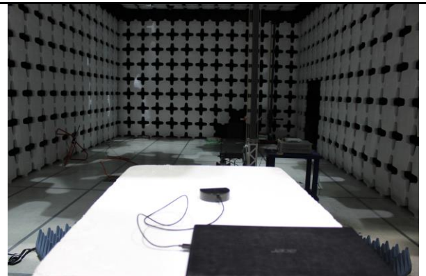
Radiated Emission Test above 1GHz Rear View
