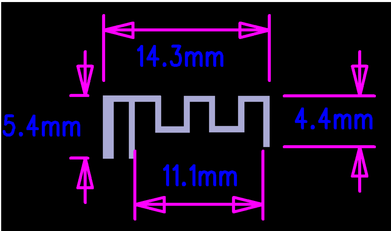
Antenna Photo & Length (mm)
