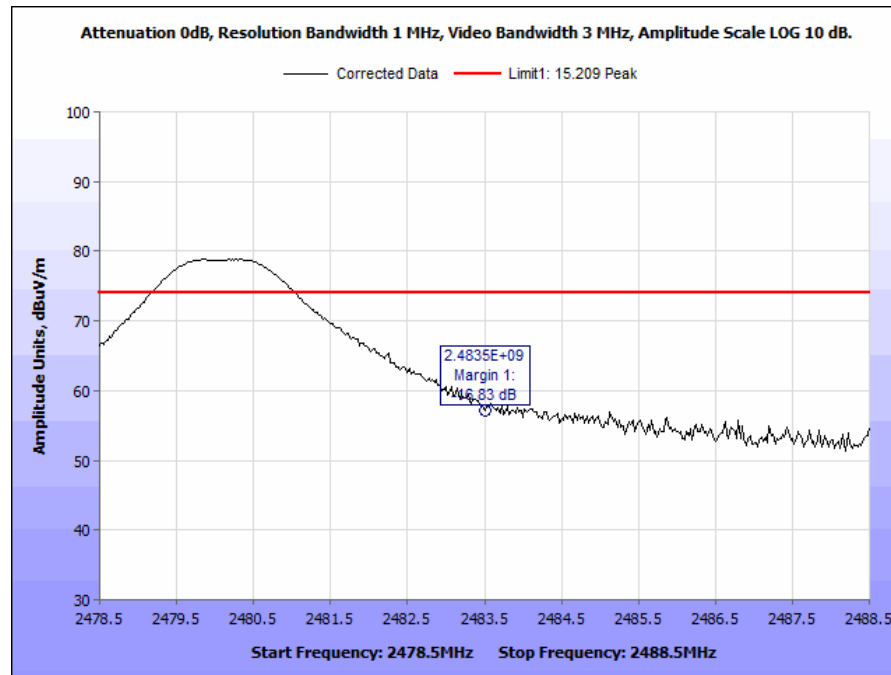
Plot 20. Radiated Band Edge, Peak, High, 2483.5 MHz, CF 2480 MHz
