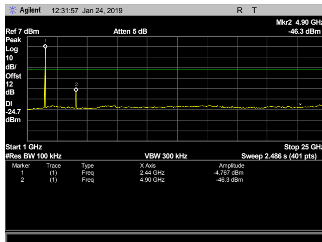
Plot 30. 100 kHz Spurious Emissions, mid channel, CF 2440M, 1 – 25 GHz
