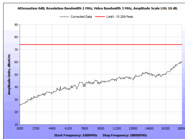
Plot 16. Radiated Emissions, Peak, CF 2440 MHz, 1 – 18 GHz
