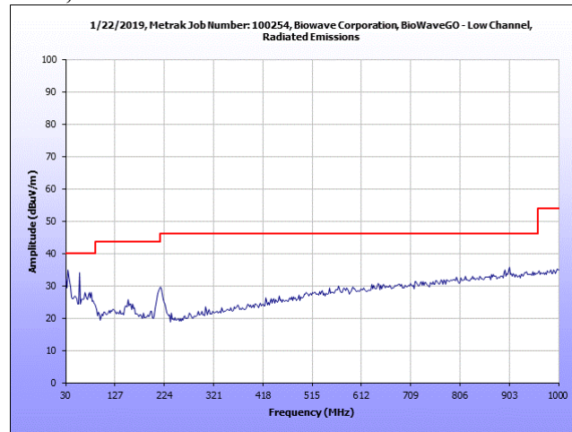
Plot 9. Radiated Emissions, Low Channel, 30 – 1000 MHz
