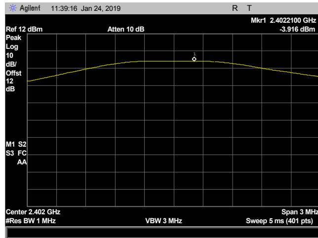
Plot 6. Peak Power Output, CF 2402 MHz
