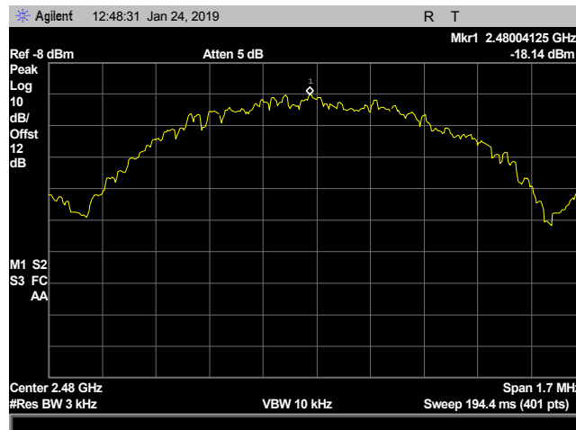
Plot 35. Power Density, CF 2480 MHz
