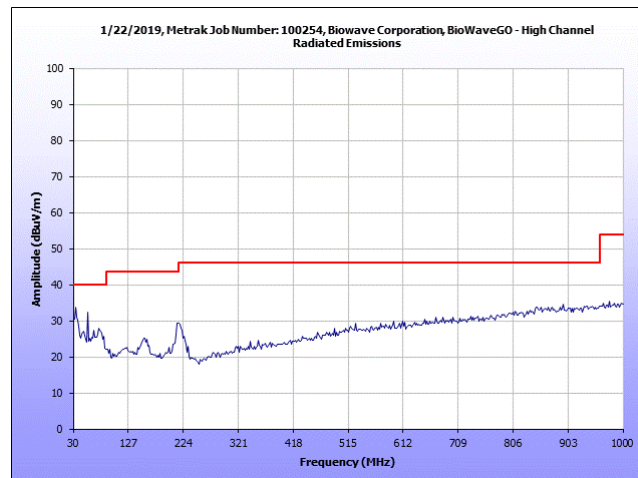
Plot 11. Radiated Emissions, High Channel, 30 – 1000 MHz
