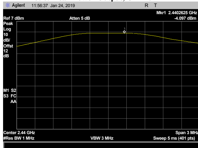
Plot 7. Peak Power Output, CF 2440 MHz
