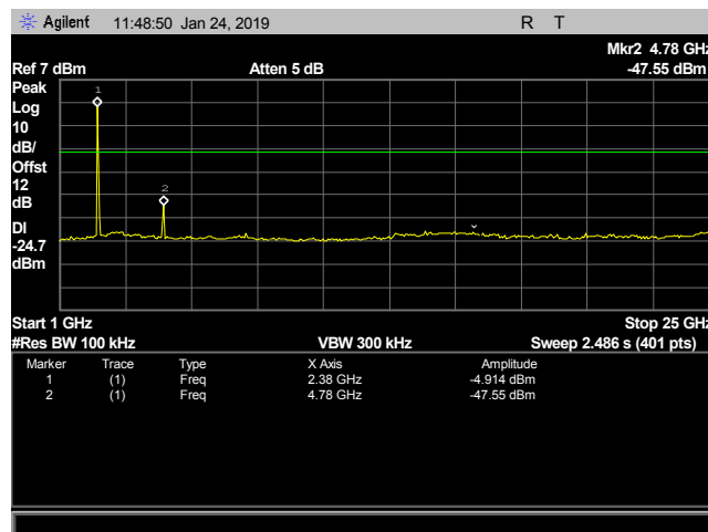
Plot 27. 100 kHz Spurious Emissions, low channel, CF 2402M, 1-25 GHz
