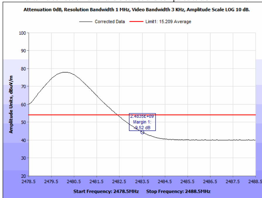
Plot 18. Radiated Band Edge, Average, High, 2483.5 MHz, CF 2480 MHz
