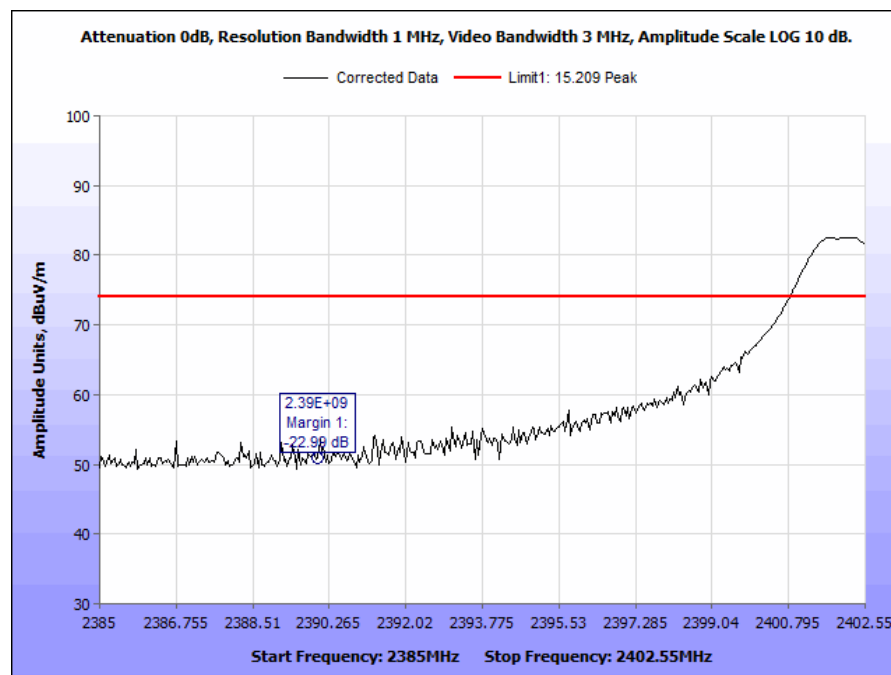
Plot 21. Radiated Band Edge, Peak, Low, 2390 MHz, CF 2402 MHz
