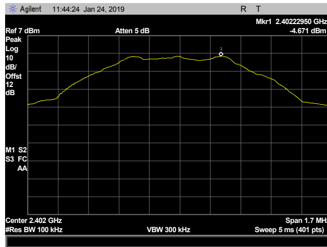
Plot 25. 100 kHz Spurious Emissions, low channel, CF 2402M, reference level
