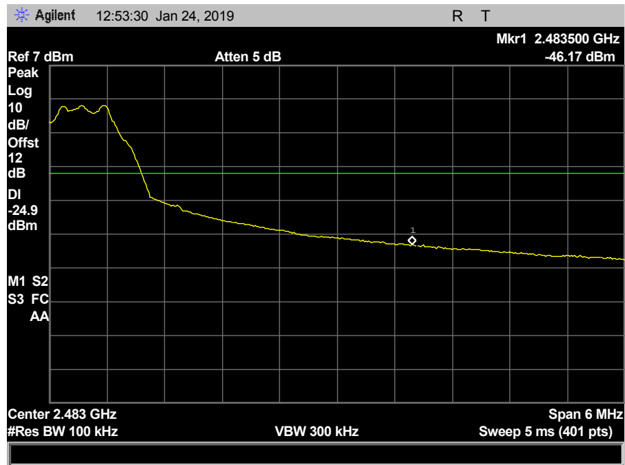
Plot 31. 100 kHz Spurious Emissions, high channel, CF 2480M, High Band Edge, 2483.5 MHz
