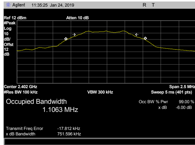
Plot 3. 6 dB Occupied Bandwidth, CF 2402
