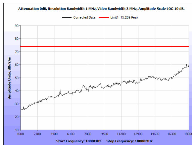
Plot 17. Radiated Emissions, Peak, CF 2480 MHz, 1 – 18 GHz
