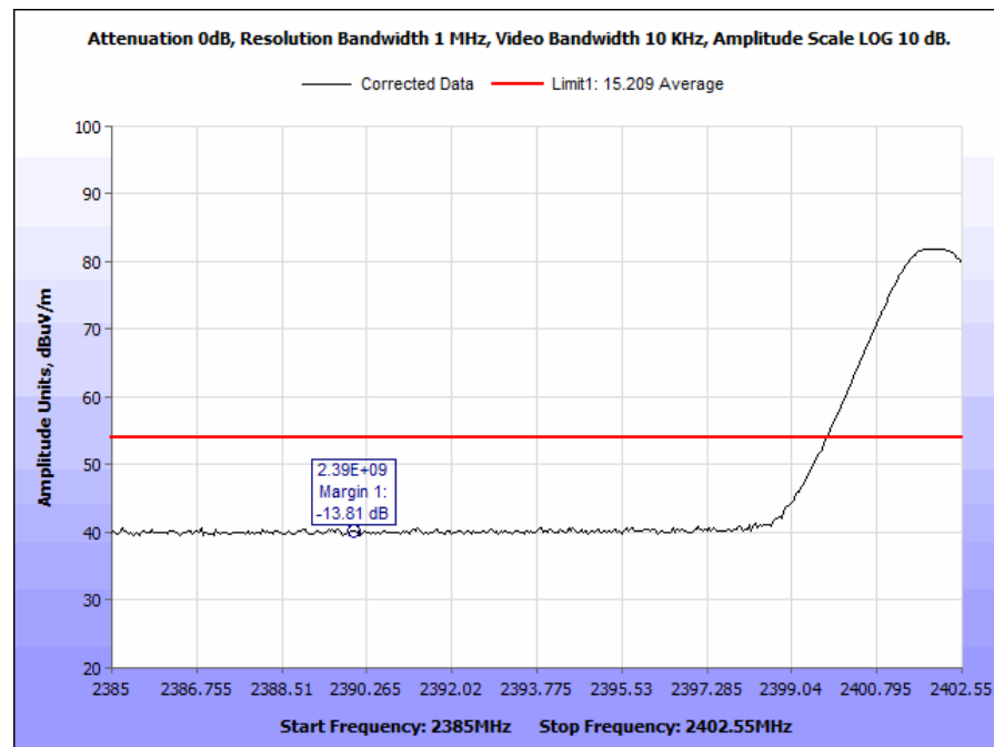
Plot 19. Radiated Band Edge, Average, Low, 2390 MHz, CF 2402 MHz
