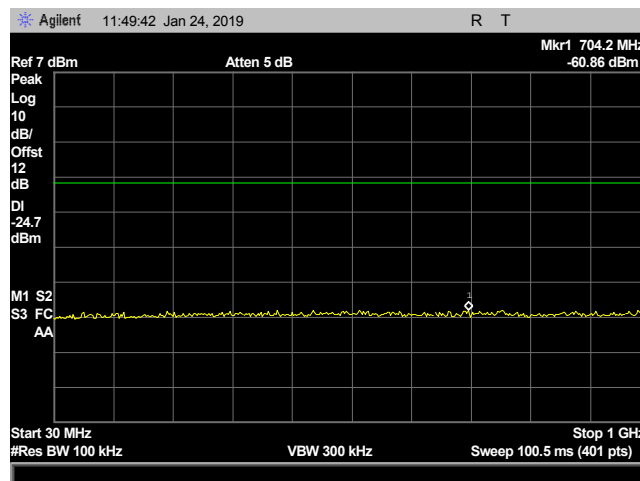
Plot 26. 100 kHz Spurious Emissions, low channel, CF 2402M, 0.03-1 GHz
