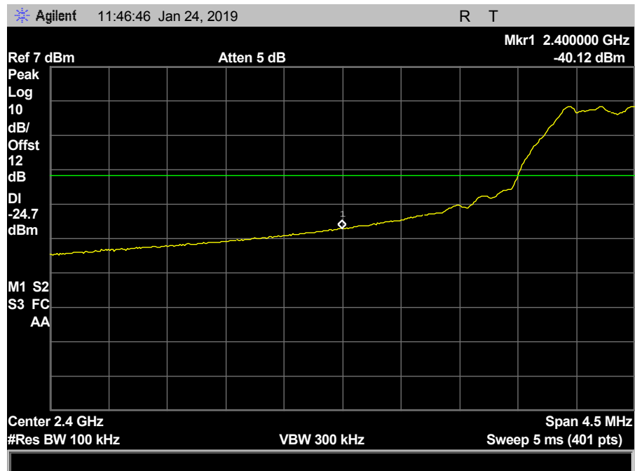
Plot 32. 100 kHz Spurious Emissions, low channel, CF 2402M, Low Band Edge 2400MHz
