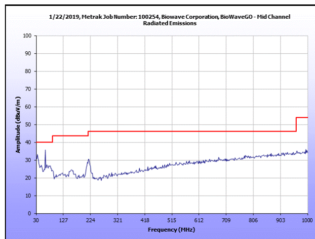
Plot 10. Radiated Emissions, Mid Channel, 30 – 1000 MHz
