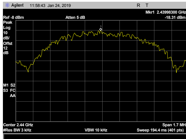
Plot 34. Power Density, CF 2440 MHz
