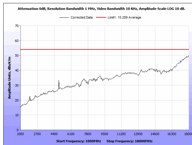
Plot 13. Radiated Emissions, Average, CF 2440 MHz, 1- 18 GHz
