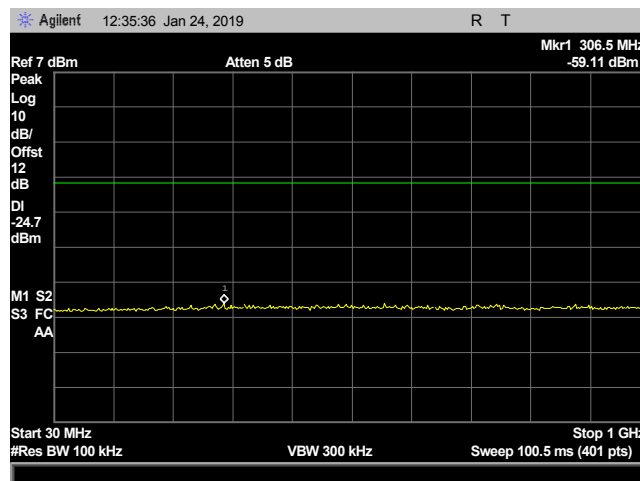
Plot 29. 100 kHz Spurious Emissions, mid channel, CF 2440M, 0.03 – 1 GHz
