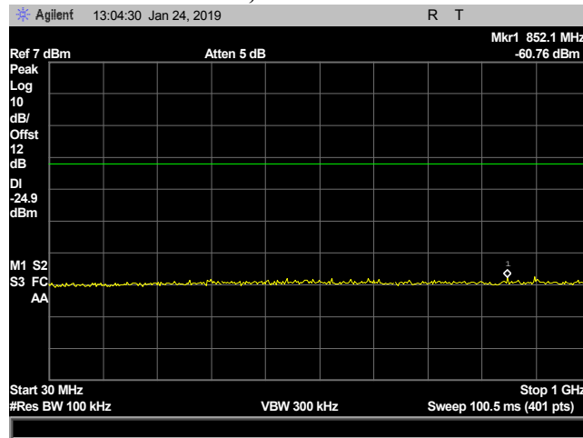
Plot 22. 100 kHz Spurious Emissions, high channel, CF 2480M, 0.03 – 1 GHz
