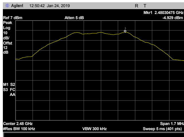
Plot 24. 100 kHz Spurious Emissions, high channel, CF 2480M, Reference Level
