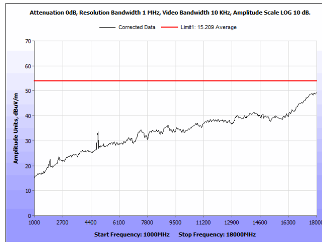
Plot 12. Radiated Emissions, Average, CF 2402 MHz, 1 – 18 GHz
