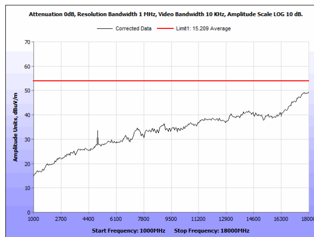
Plot 14. Radiated Emissions, Average, CF 2480 MHz, 1 – 18 GHz
