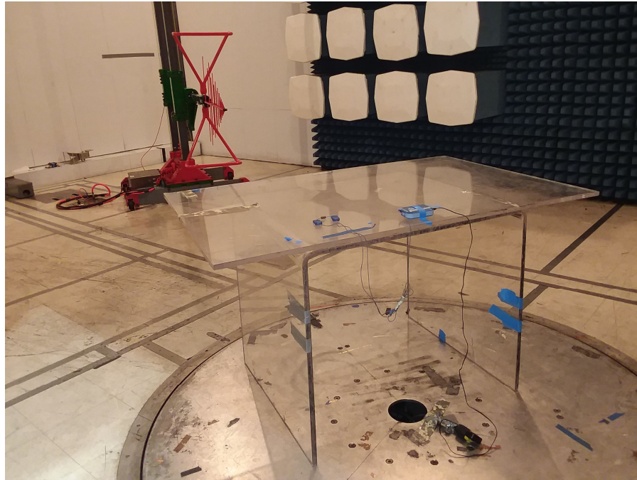
Photograph 2. Radiated Emissions, Setup Below 1GHz
