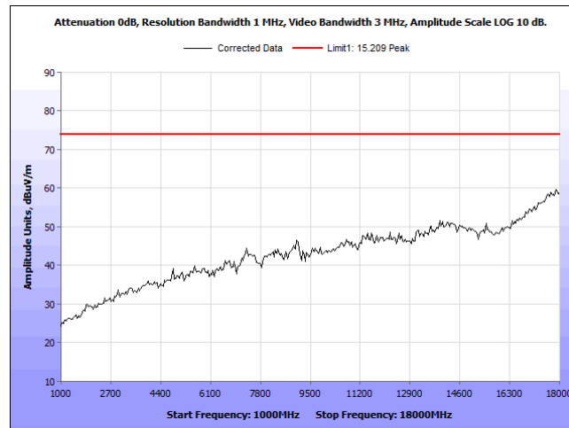
Plot 15. Radiated Emissions, Peak, CF 2402 MHz, 1 – 18 GHz
