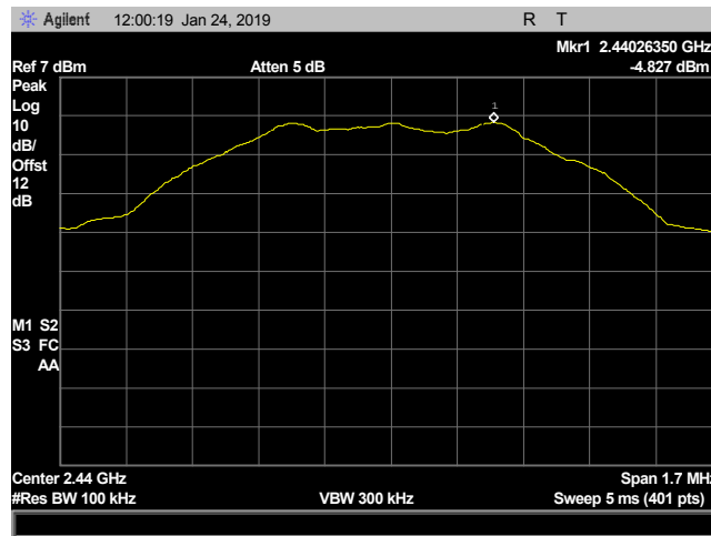
Plot 28. 100 kHz Spurious Emissions, mid channel, CF 2440M, reference level
