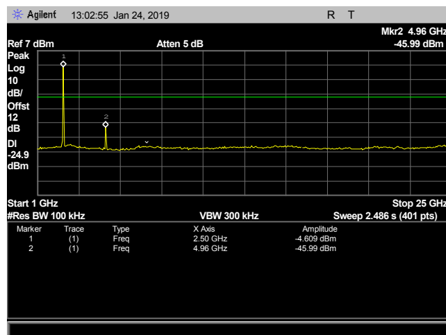
Plot 23. 100 kHz Spurious Emissions, high channel, CF 2480M, 1 – 25 GHz
