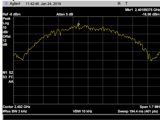
Plot 33. Power Density, CF 2402 MHz
