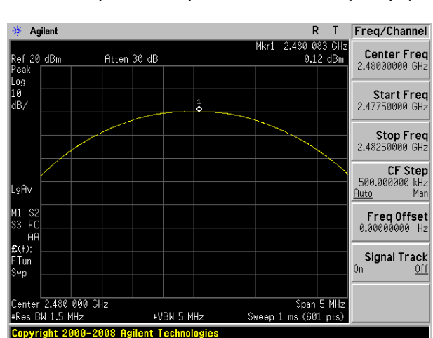
Peak output Power plot on channel 78 (2Mbps)
