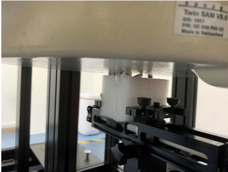
Front Side (0mm) of Right Headset
