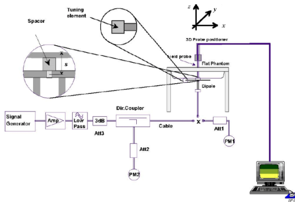
Fig.7.1 System Verification Setup Diagram
