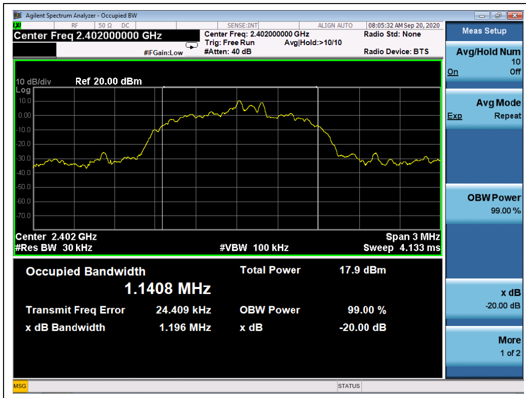
(Channel 0, 8-DPSK)
