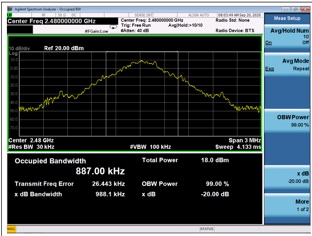
(Channel 78, GFSK)
