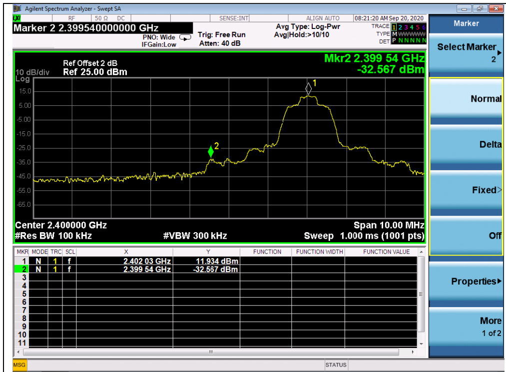
(Band edge, Channel 0, \pi/4 -DQPSK)
