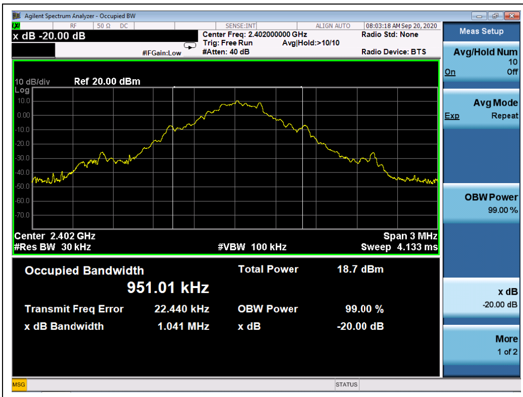
(Channel 0, GFSK)
