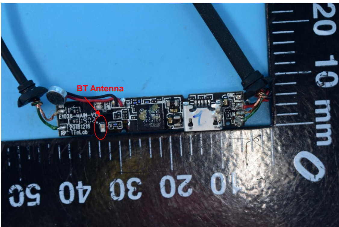
2. Antenna view
