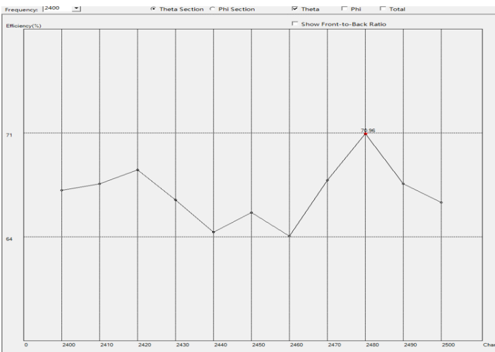
2400-2500MHZ Efficiency
