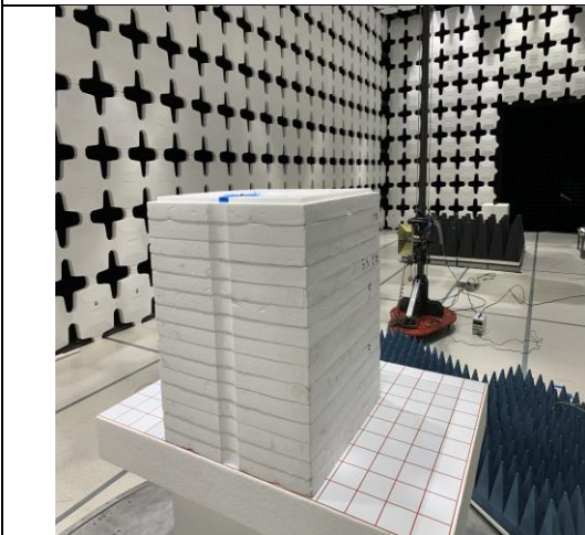
RSE-Above 1GHz-Back
