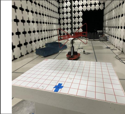
RSE-Below 1GHz-Back
