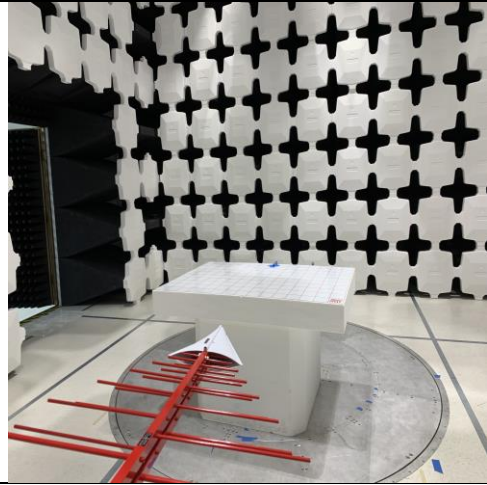
RSE-Below 1GHz-Front
