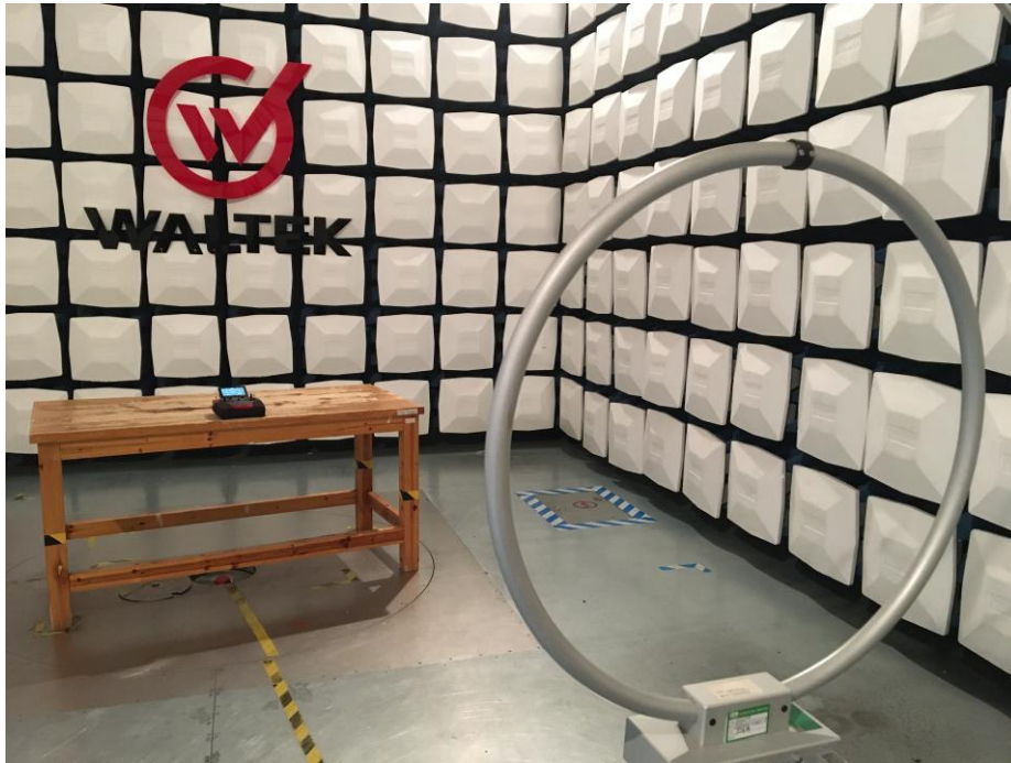
Test Setup For Radiated Emission (Below 30MHz)
