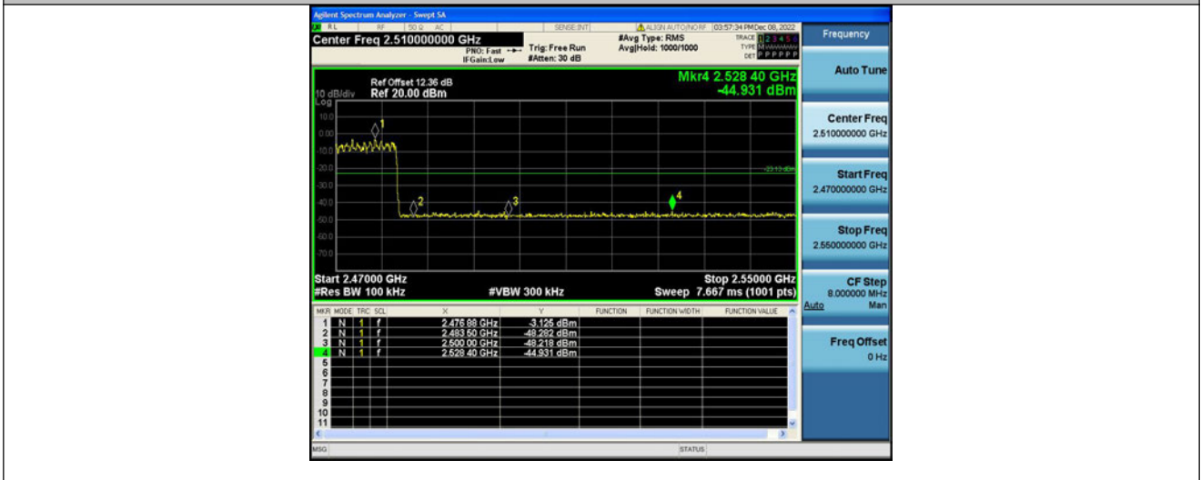
3DH5-Ant1-High-Hop_2480-3.13
