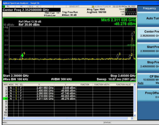
3DH5-Ant1-Low-2402--2.08
