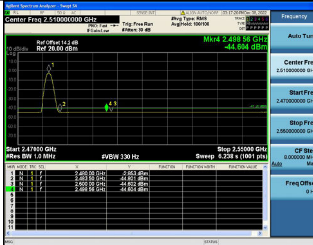
3DH5-Ant1-High-2480-Peak-2483.500
