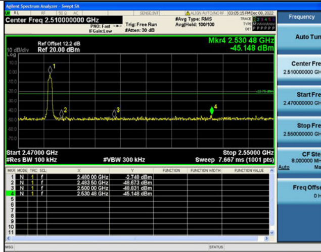
3DH5-Ant1-High-2480-1.85
