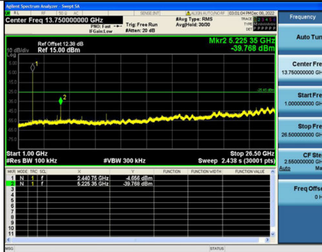
3DH5-Ant1-2441-0-Reference-5.34
