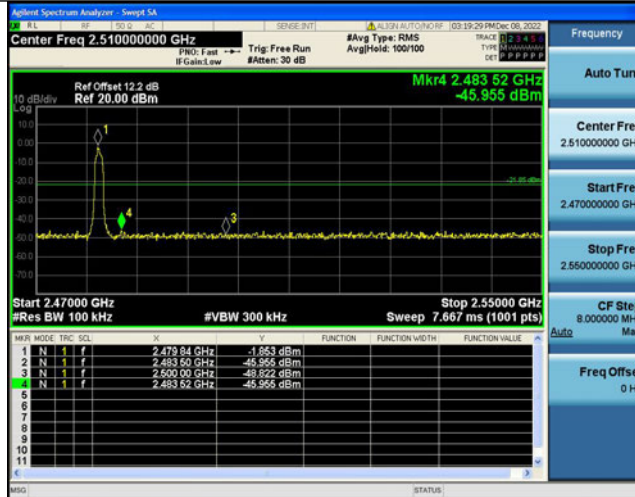
DH5-Ant1-Low-Hop_2402-2.68
