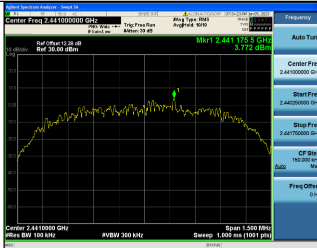
3DH5-Ant1-2441-30-1000-3.77
