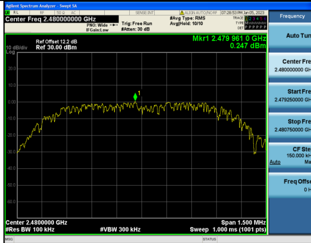
2DH5-Ant1-2480-30-1000-0.25
