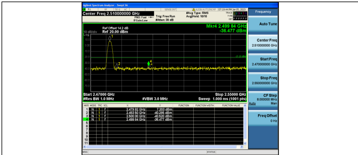
DH5-Ant1-High-2480-AV-2483.500
