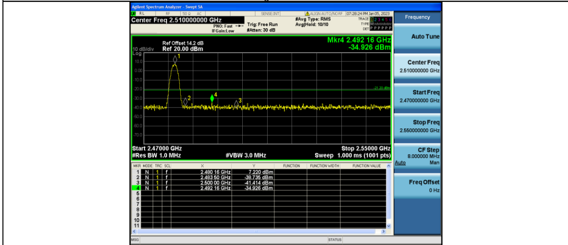
2DH5-Ant1-High-2480-AV-2483.500
