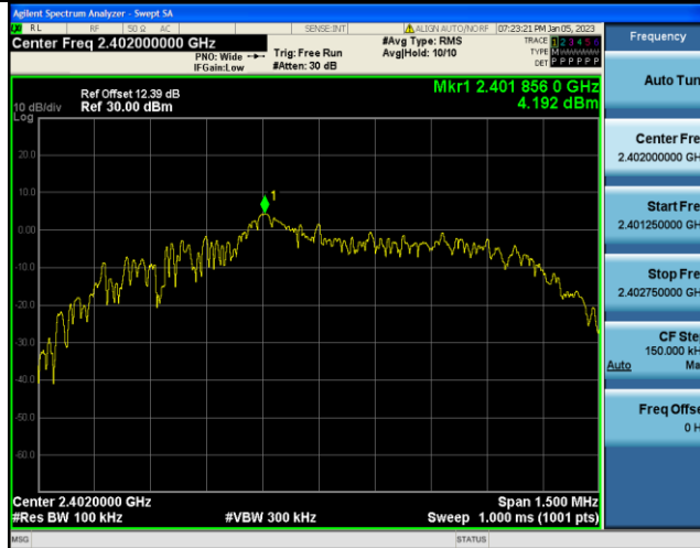
2DH5-Ant1-2402-30-1000-4.19
