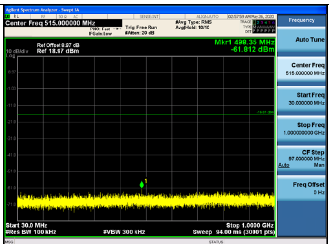
\pi/4 -DQPSK on Channel 78
