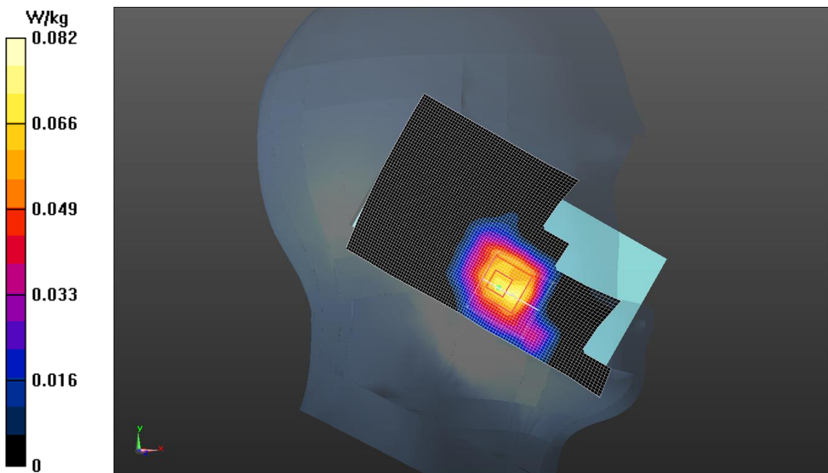
Fig.11 LTE Band 2
