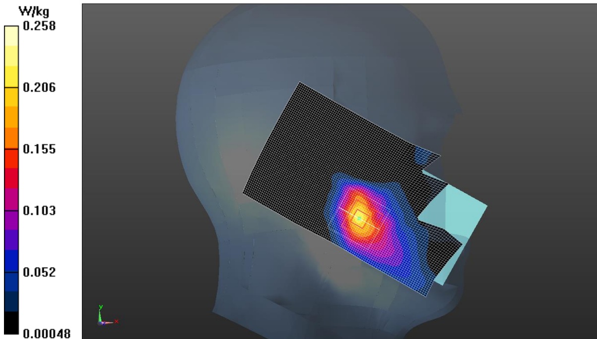
Fig.17 LTE Band 7
