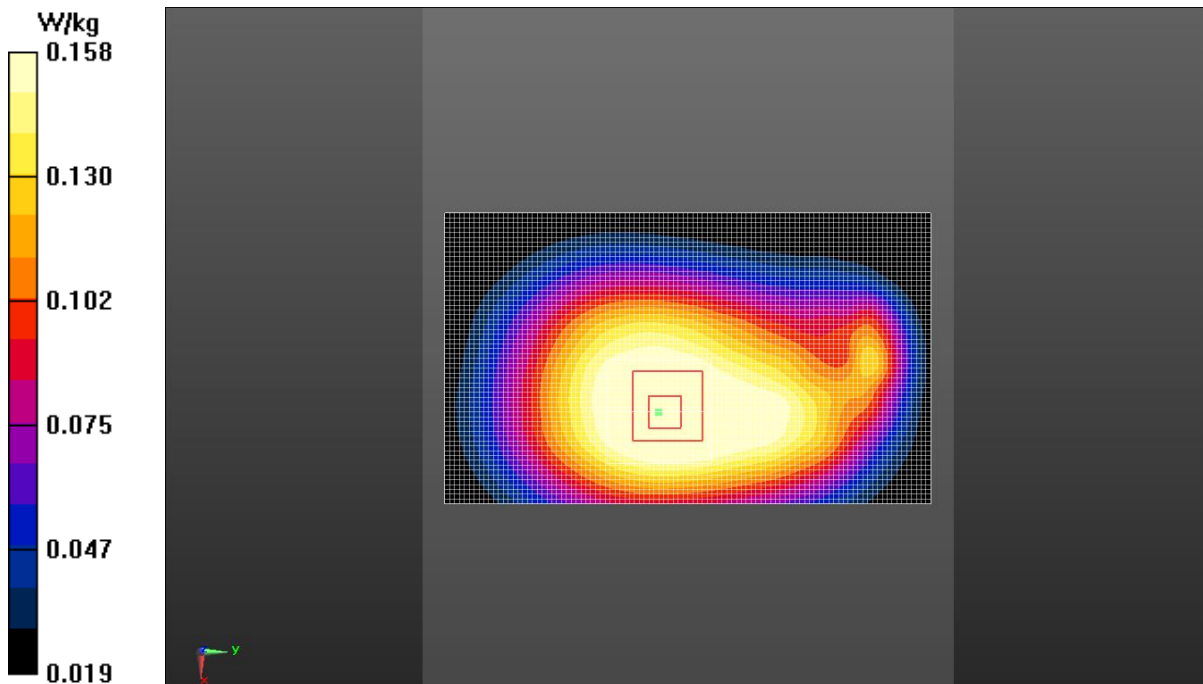
Fig.16 LTE Band 5
