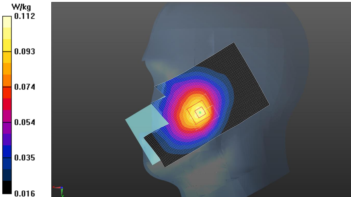
Fig.15 LTE Band 5
