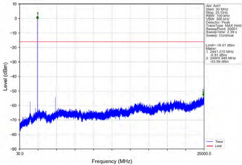
Pi/4DQPSK_2DH5_MCH_2441MHz_Ant1 NTN
