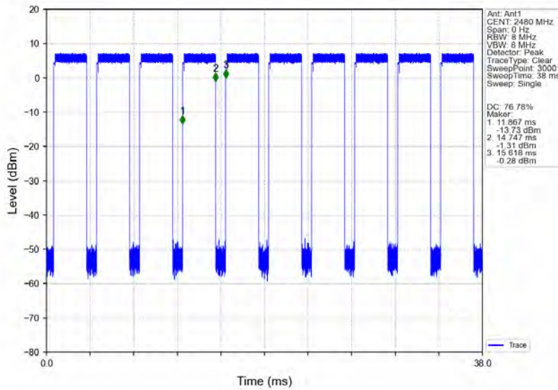
Pi/4DQPSK_2DH5_HCH_2480MHz_Ant1_NTNV
