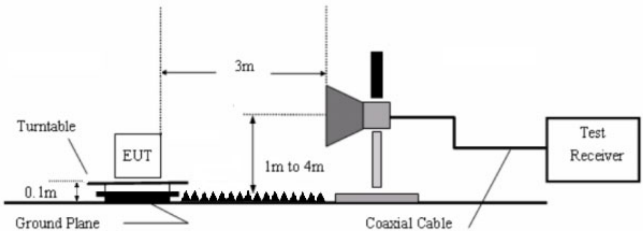
Figure 3. Above 1 GHz
