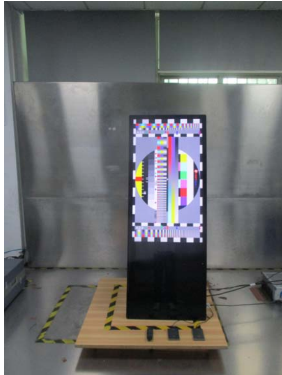
Conducted Emissions Side View DGSNAFNT43
