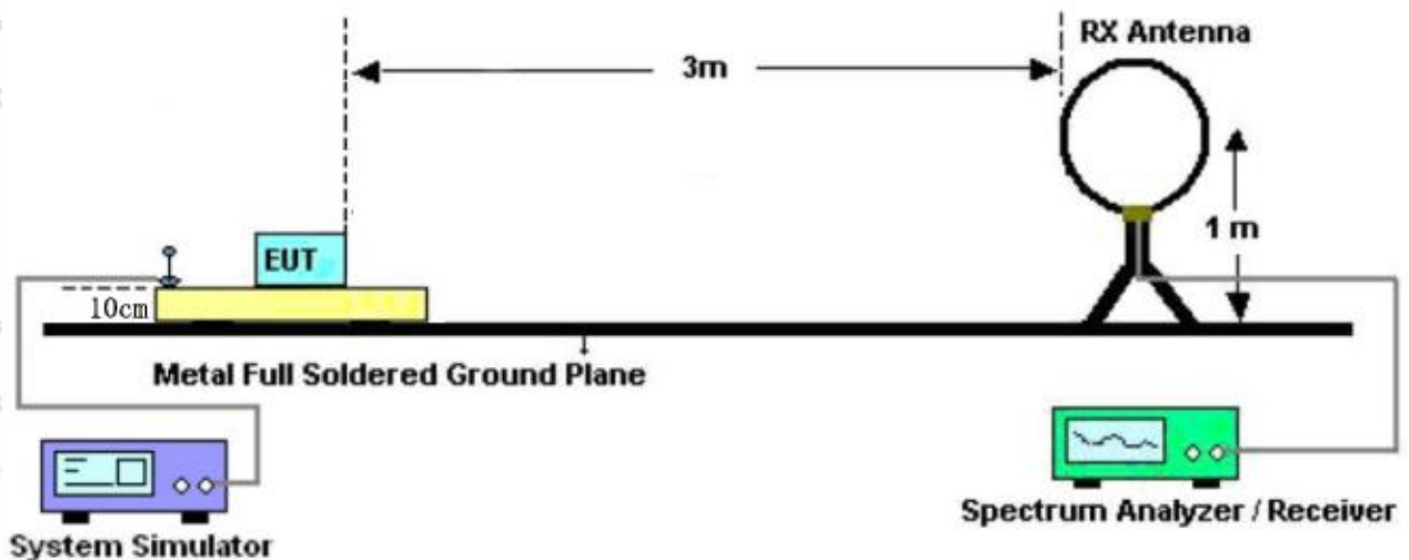
Figure 1. Below 30MHz
