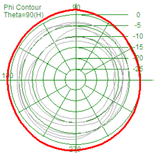
Gain: 4.85dBi
