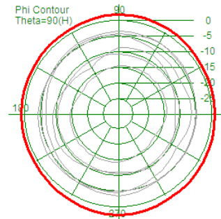
Gain: 4.83dBi
