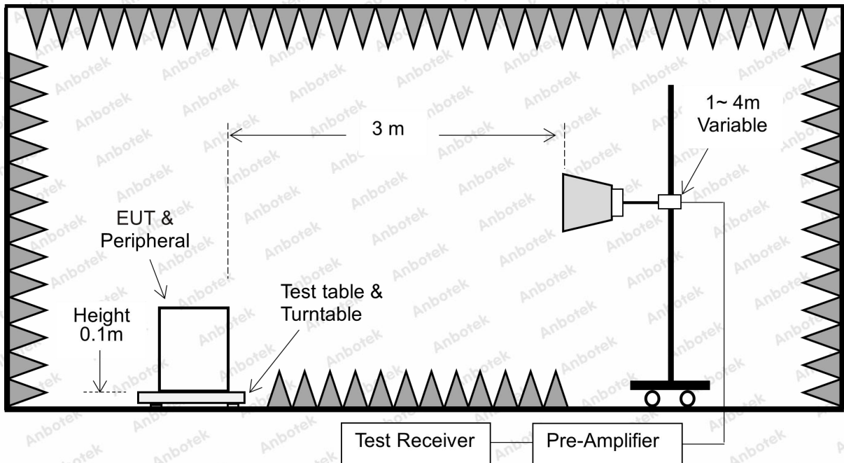
Figure 3. Above 1 GHz
