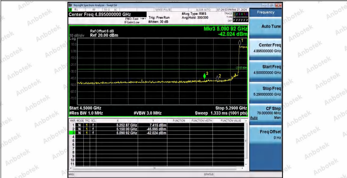
11AX40SISO_Ant1_High_5310
