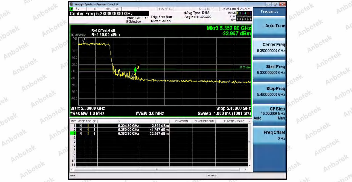
11AX40SISO_Ant1_High_5310
