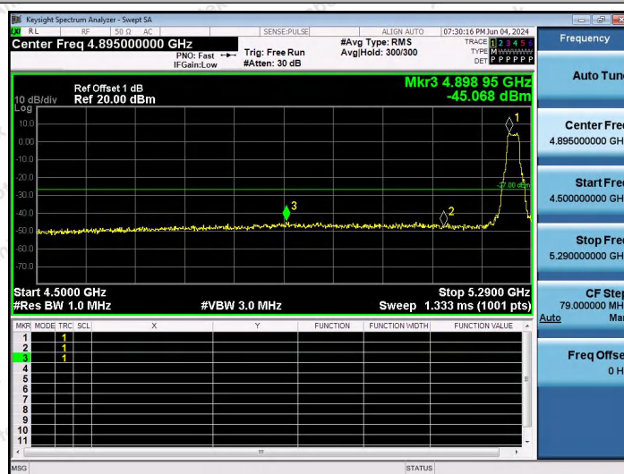
11AC20SISO-Ant1-5260-PASS
