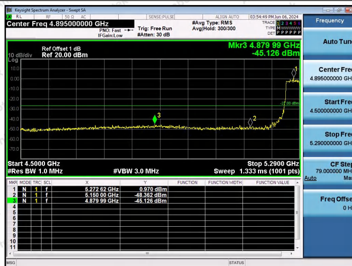
11AX40SISO-Ant1-5270-PASS
