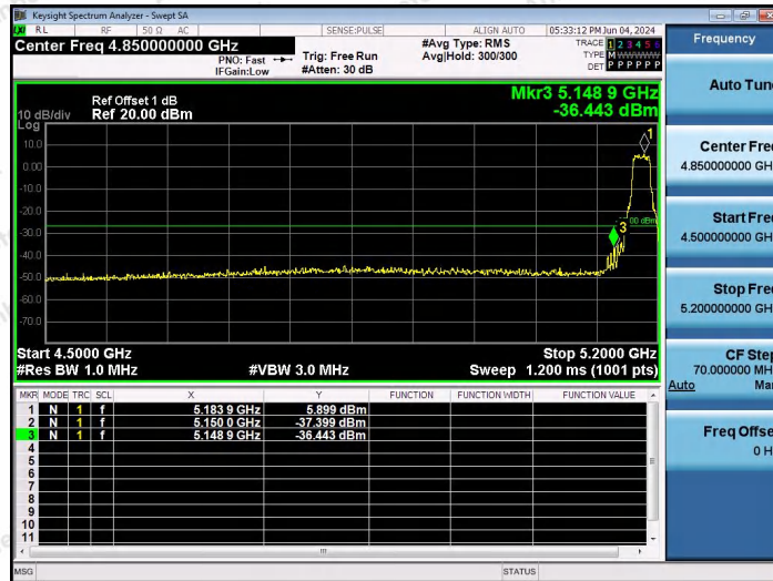
11AX20SISO-Ant1-5180-PASS
