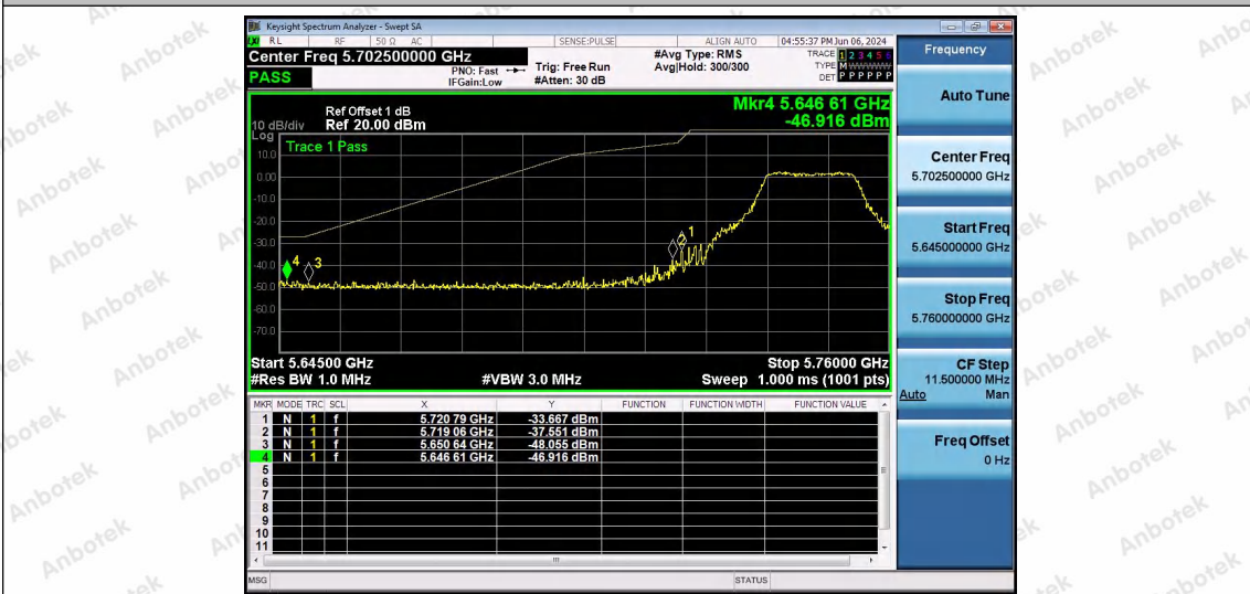
11N20SISO-Ant1-5745-PASS
