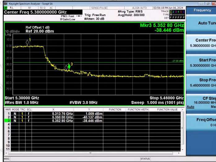
11AX40SISO-Ant1-5310-PASS
