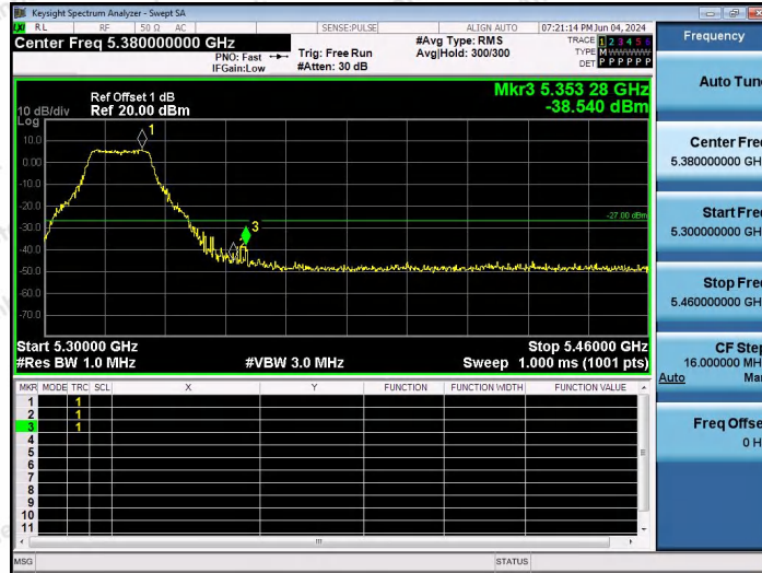
11A-Ant1-5320-PASS
