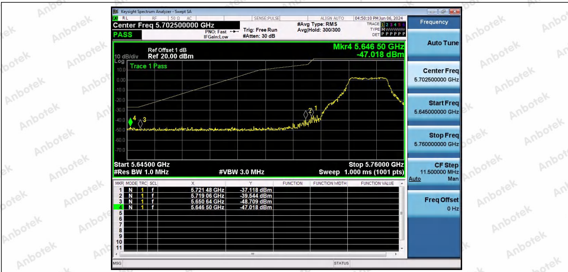
11A-Ant1-5745-PASS
