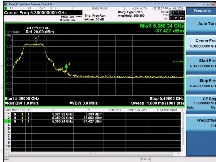
11AX20SISO-Ant1-5320-PASS
