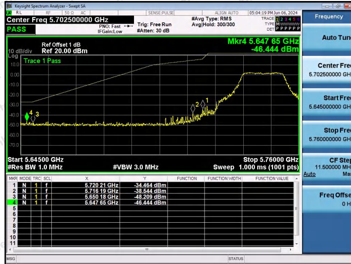
11AC20SISO-Ant1-5745-PASS
