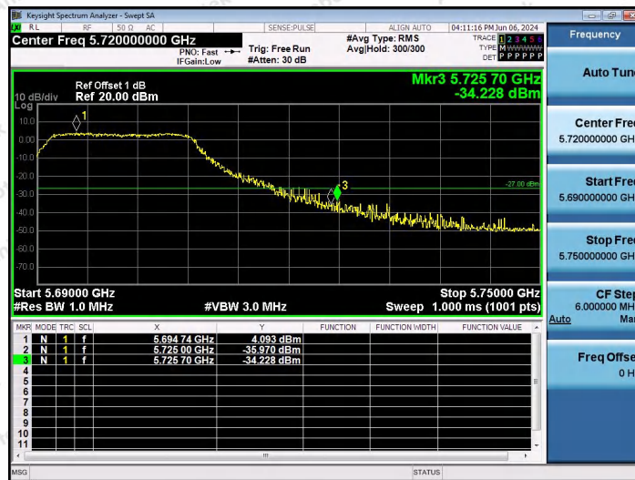
11N20SISO-Ant1-5700-PASS
