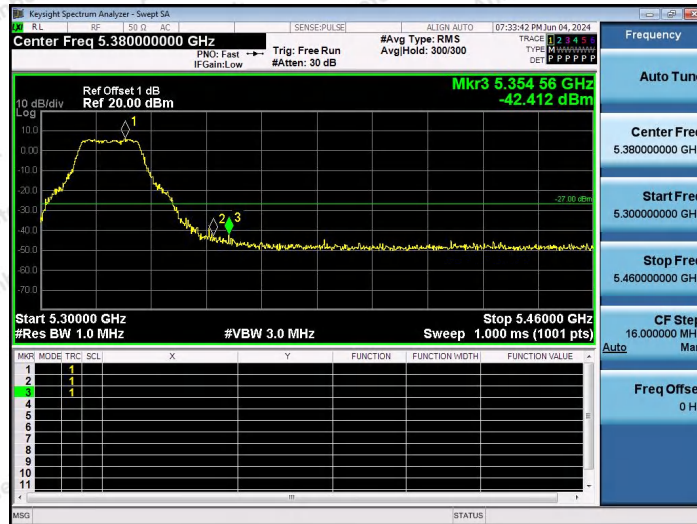
11AC20SISO-Ant1-5320-PASS
