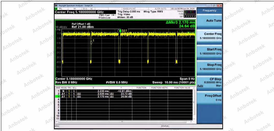
NTNV-11A-Ant1-5180
