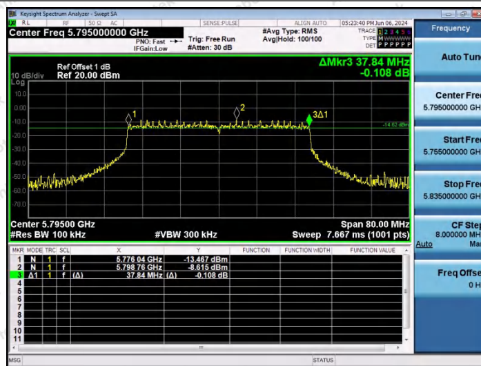
11AX40ISO-Ant1-5795-PASS
