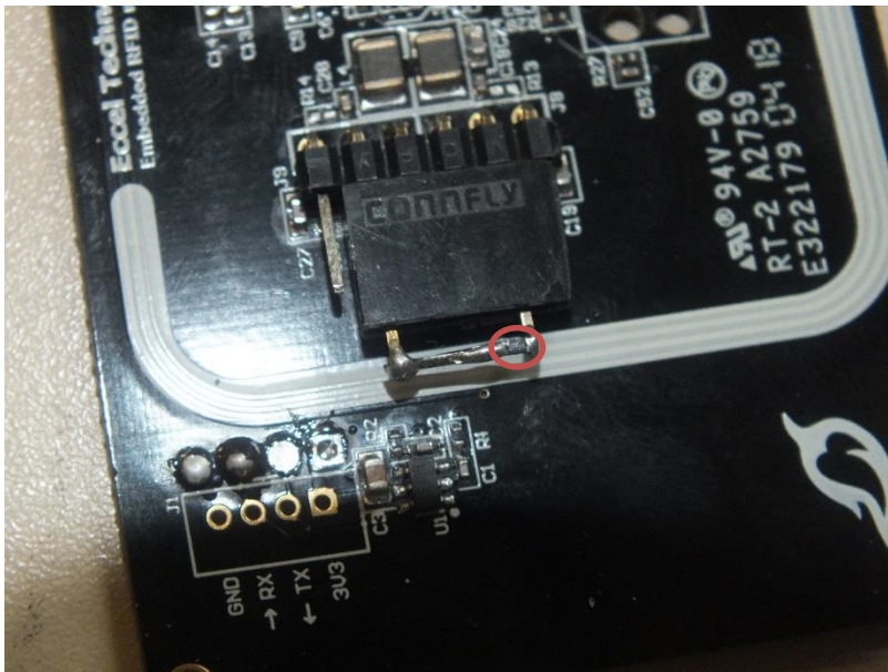
RED circle: Resistor for termination
