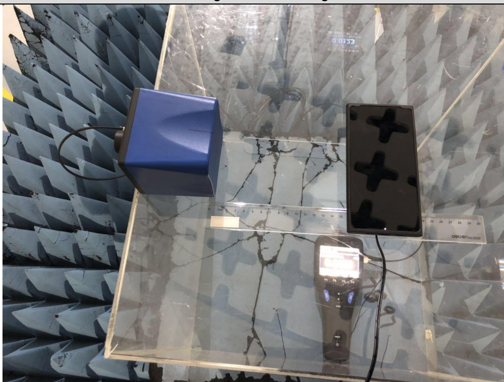
E-Field Strength/H-Field Strength 15cm
