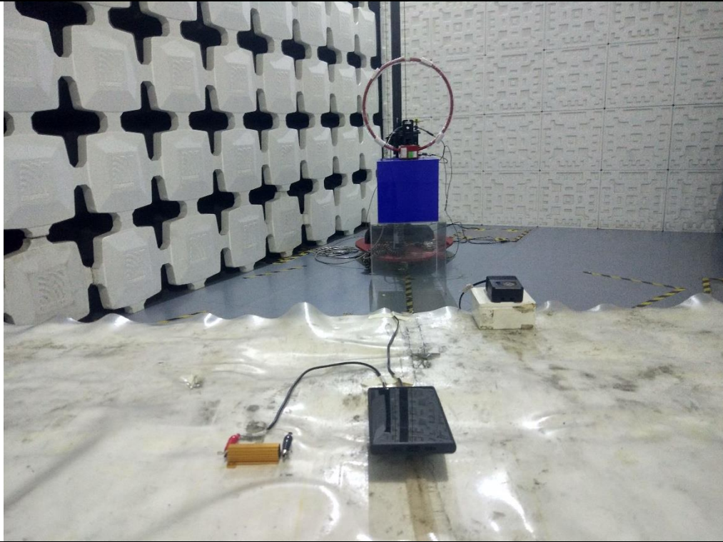
Radiated emission Test Setup (Below 30MHz)
