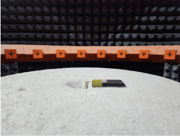
Test Setup Front View
