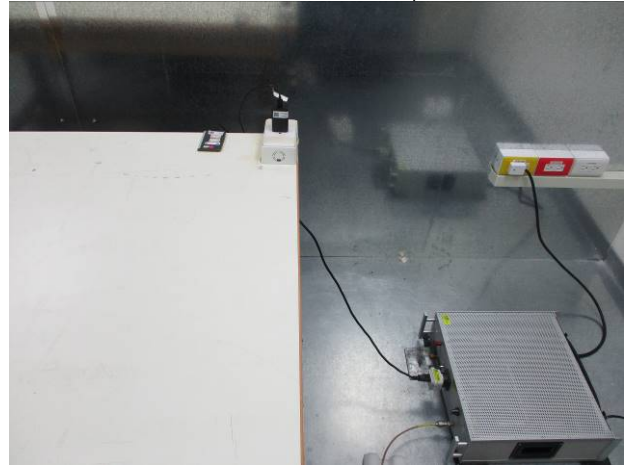
NFC_Conduction_Setup
