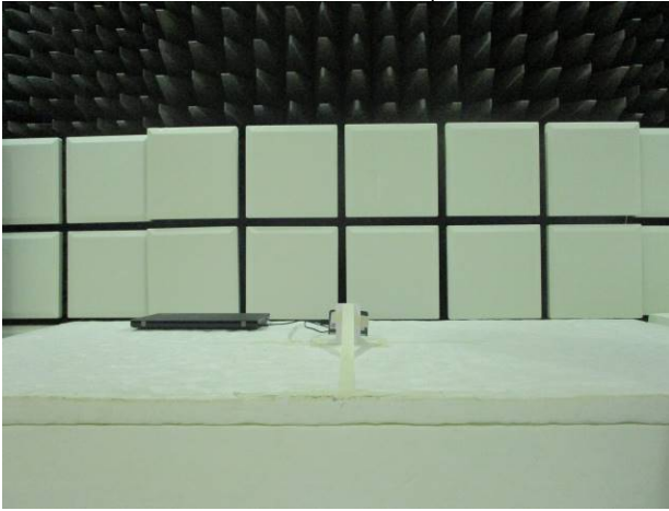
NFC_Radiated_Setup
