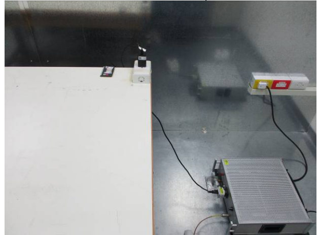
LE_Conduction_Setup
