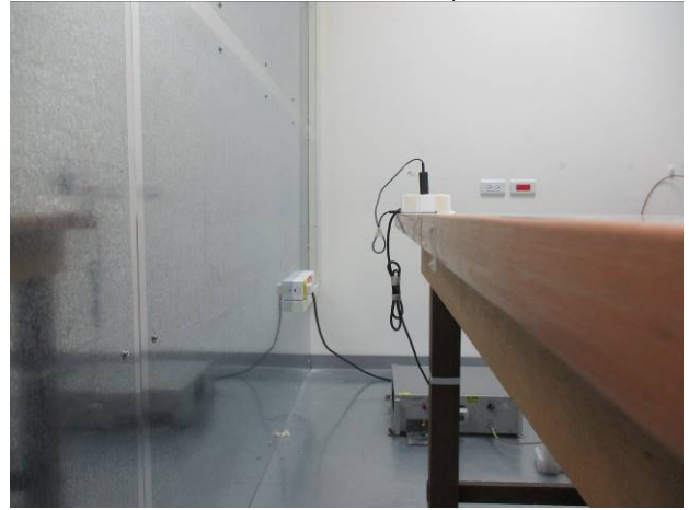
NFC_Conducted_Setup.png
