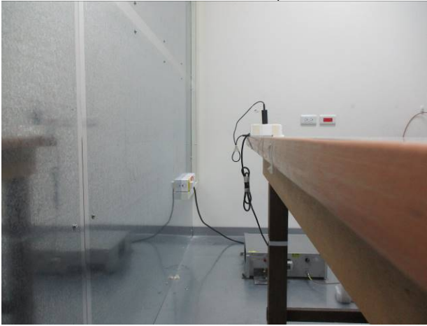
LE_Conduction_Setup
