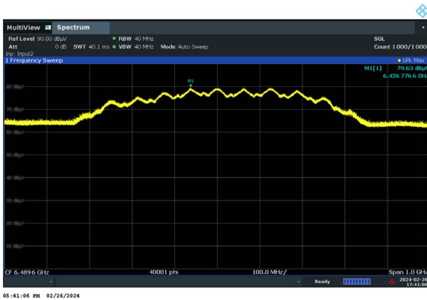
6 489.6 MHz & X axis & Hor
