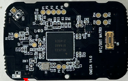
Chip Antenna
