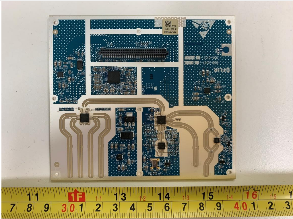
EUT Radar – PCBA2 Top View
