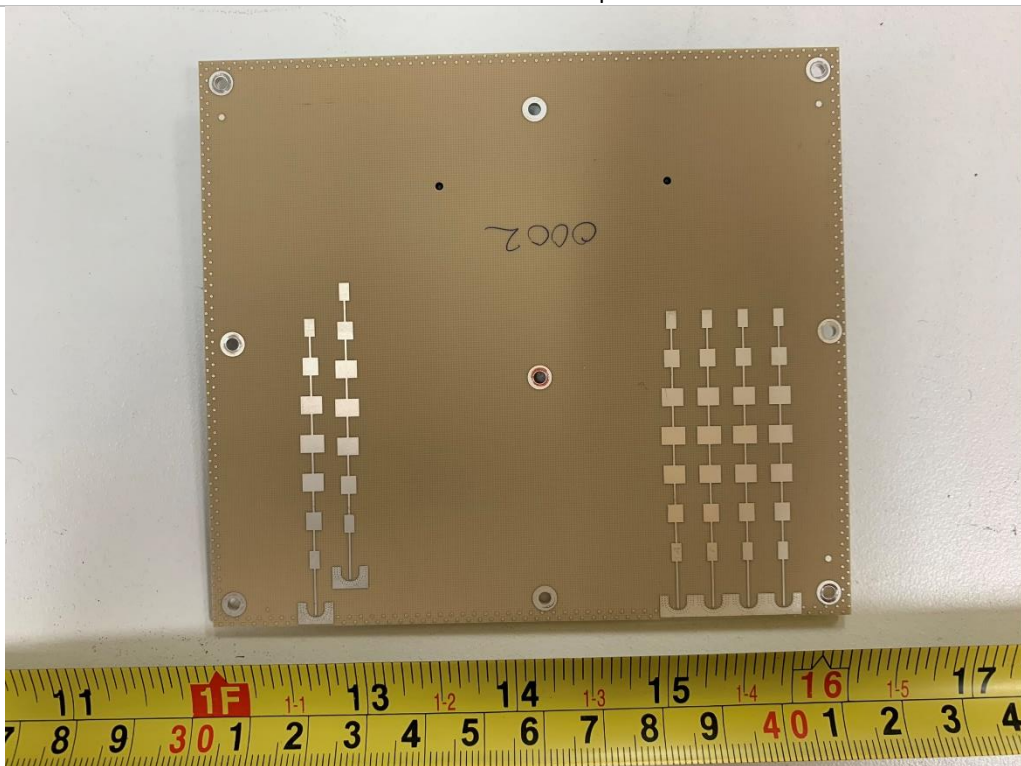
EUT Radar – PCBA2 Bottom View
