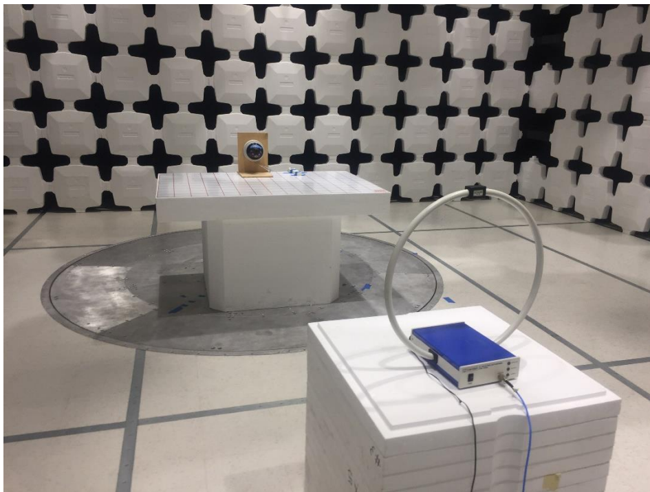
Radiated Emissions Below 30MHz setup – Front
