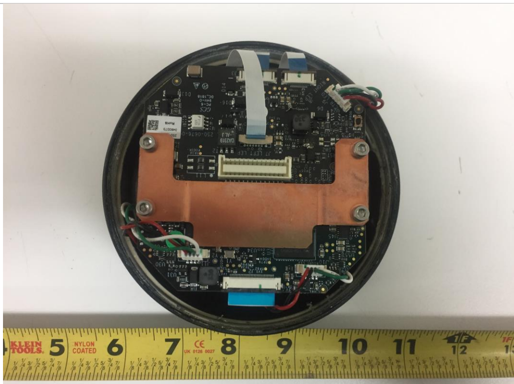
EUT Cover Off View-2
