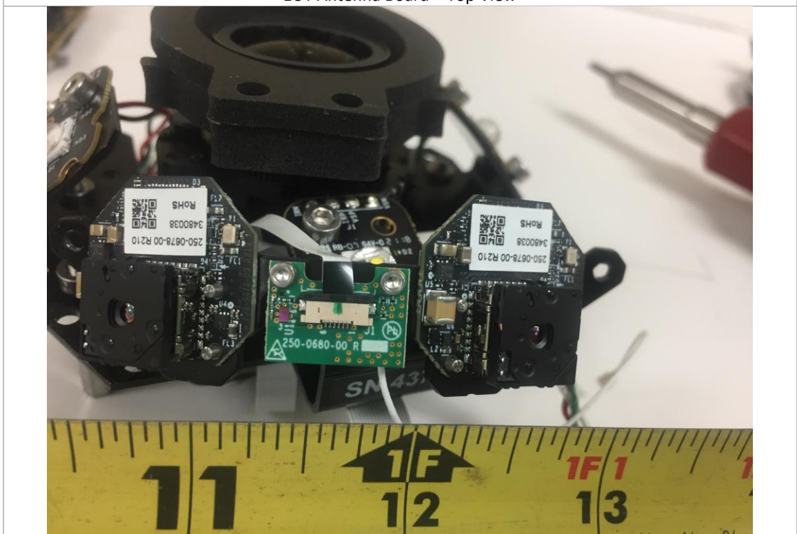
EUT Antenna Board – Bottom View
