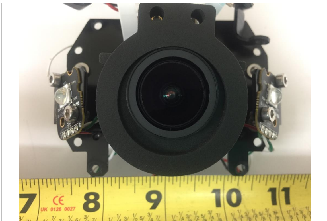
EUT Cover Off View-3
