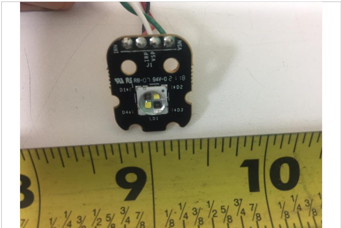
EUT PCB3 – Top View
