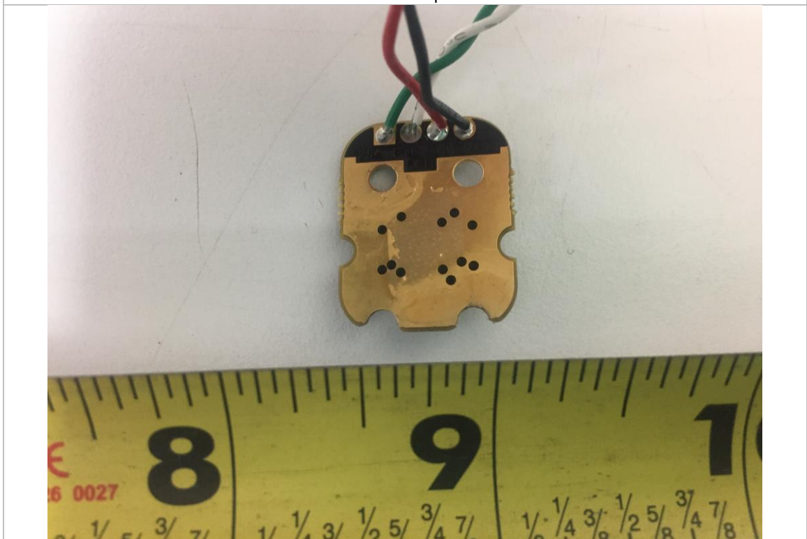
EUT PCB3 – Bottom View
