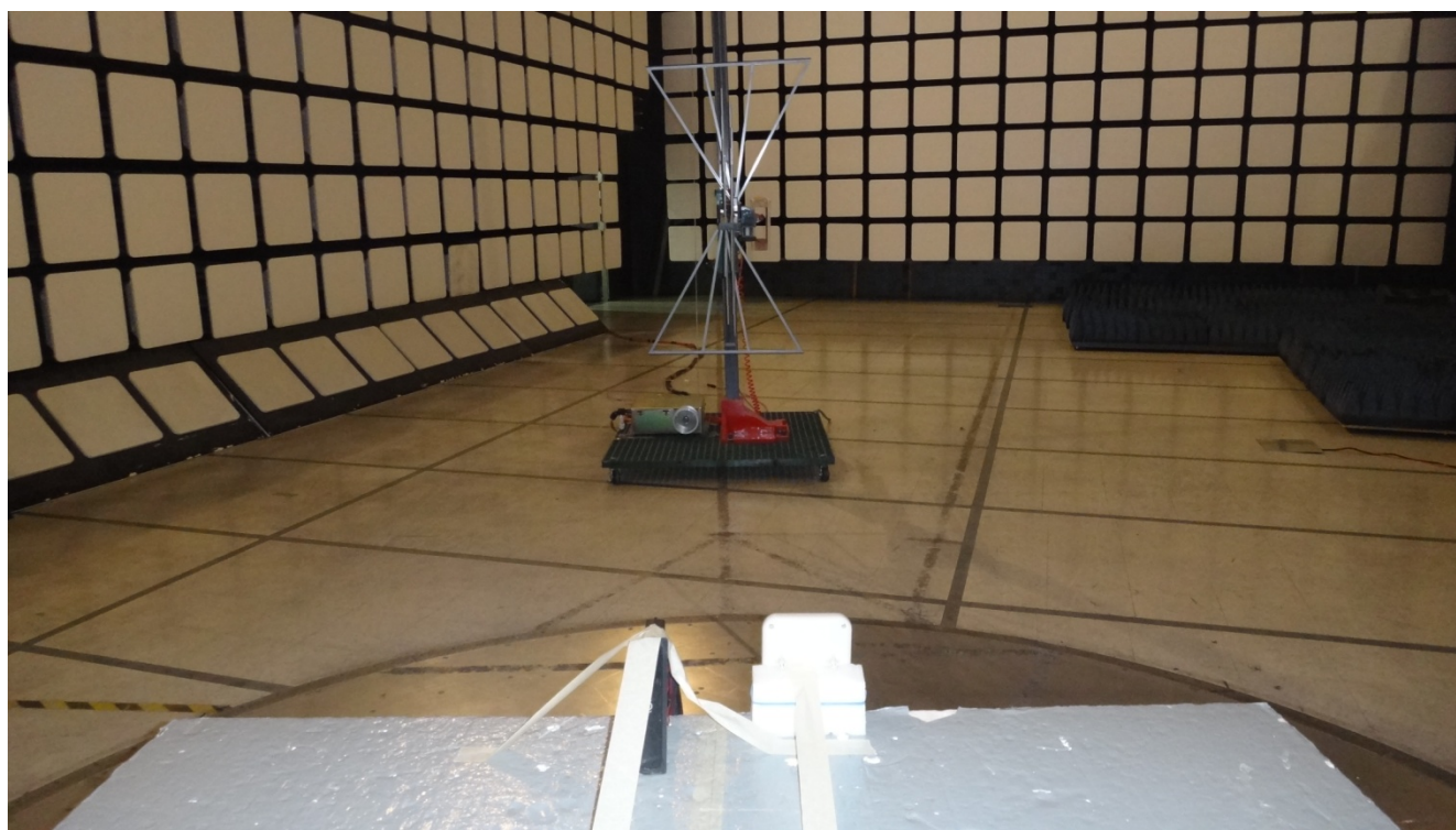
Radiated Emissions @ 3 m, Orthogonal Position 2
