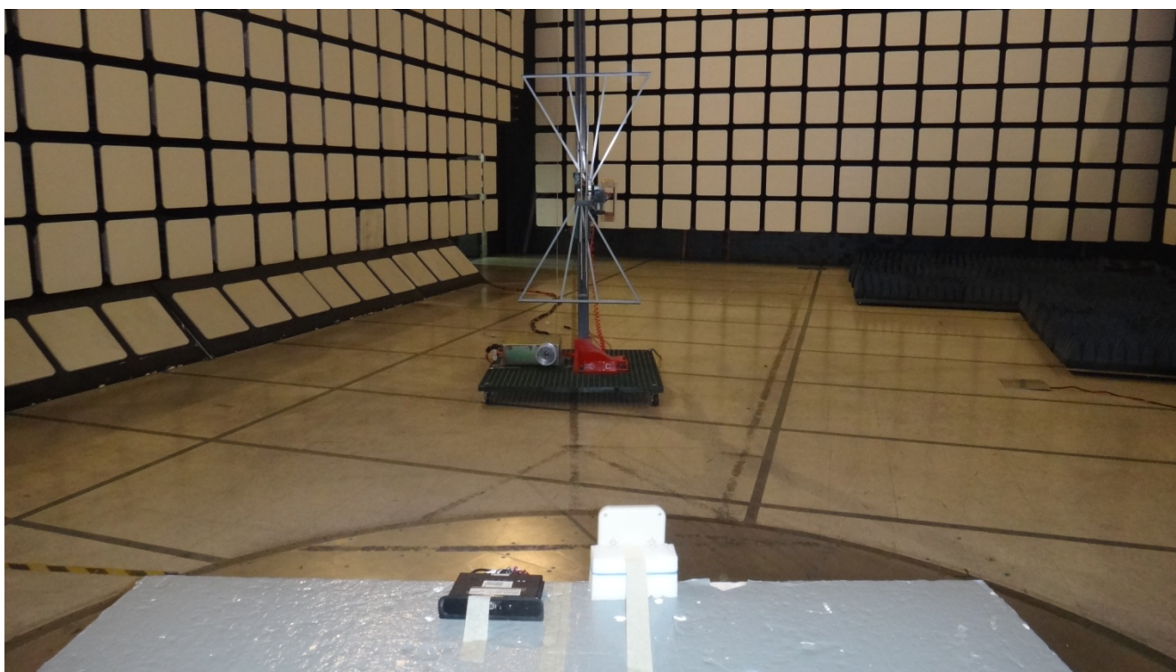
Radiated Emissions @ 3 m, Orthogonal Position 1
