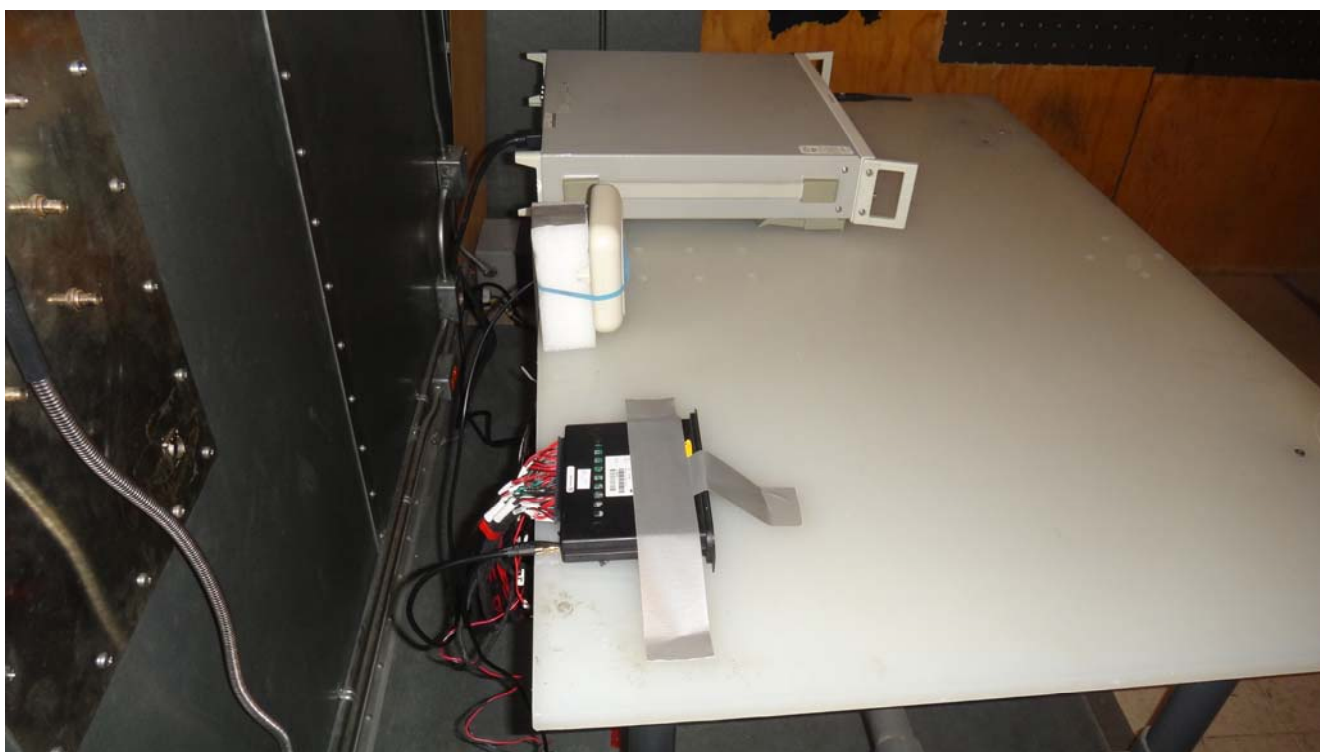
Power Line Conducted Emissions
