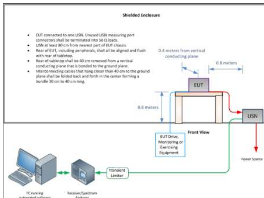
Figure 3 - Test Setup
