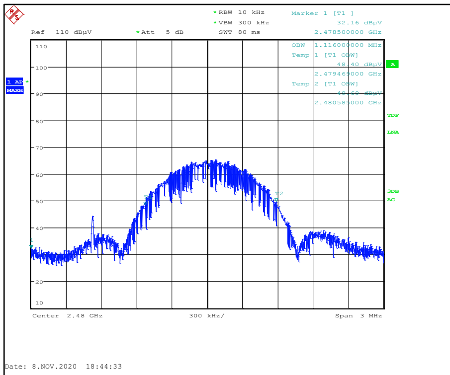
Figure 11 - 2480 MHz – 99% Occupied Bandwidth
