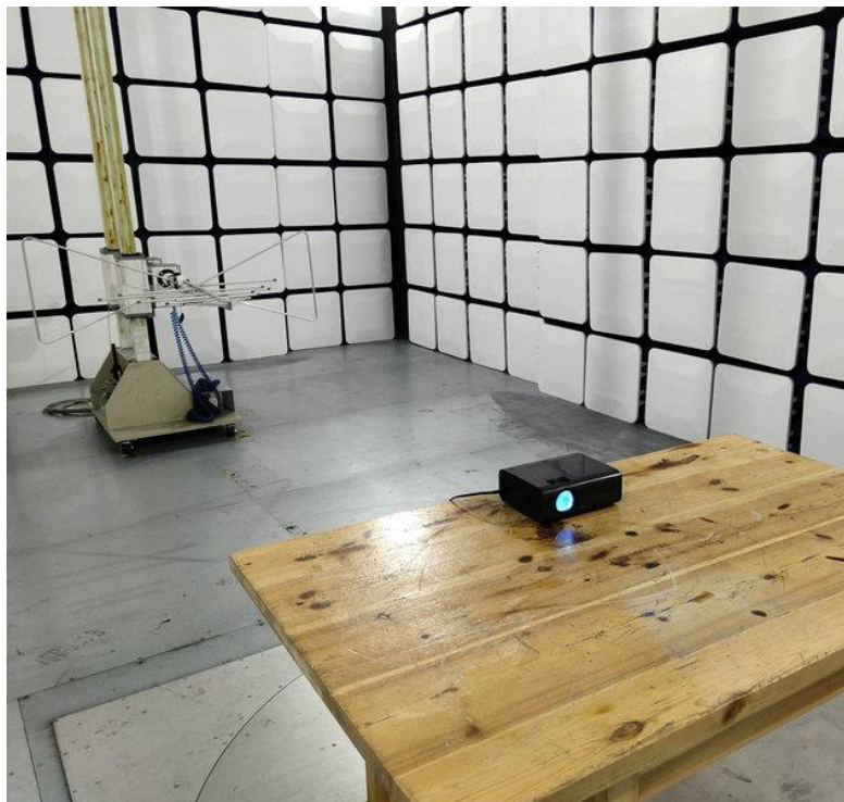
Photo of Radiation Emission Test
