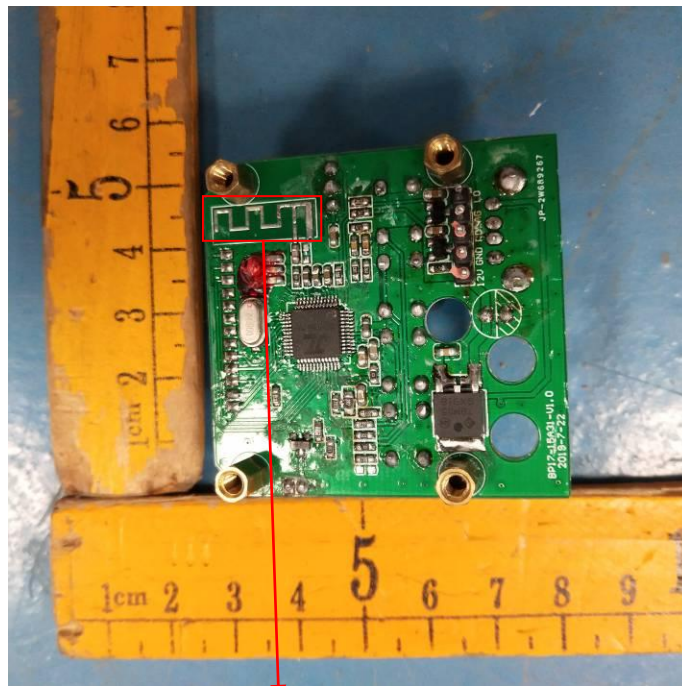
RF Antenna
