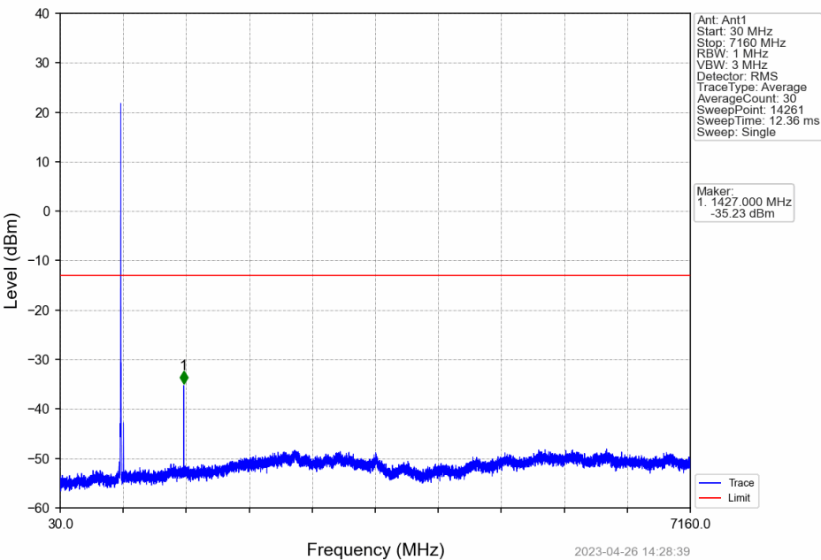
Band12 3MHz QPSK HCH 714.5MHz RB 1 14 NTN
