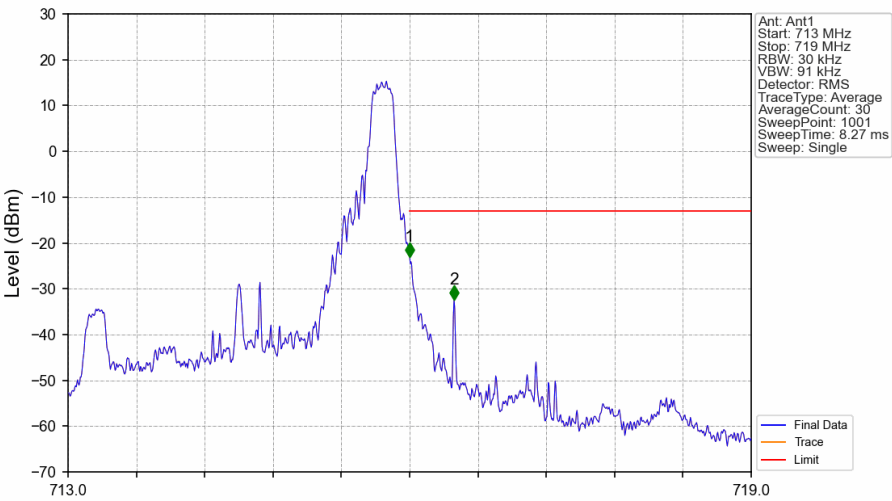
Band12 3MHz QPSK HCH 714.5MHz RB 1 14 NTN
