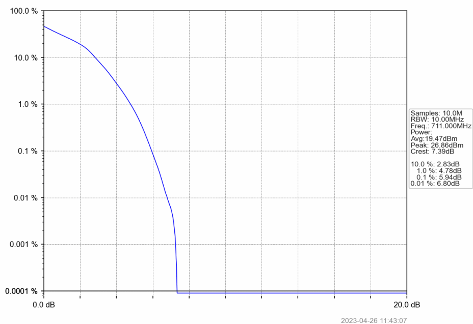
Band12 10MHz 16QAM HCH 711MHz RB 50 0 NTN
