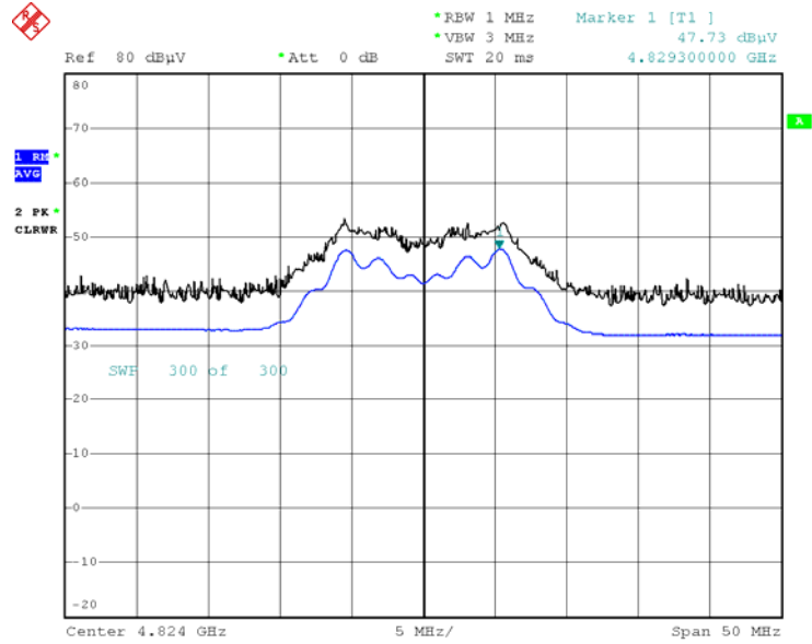
Radiated Spurious Emissions plot – Average Reading (802.11b_1Mbps, Ch.1 2nd Harmonic)
