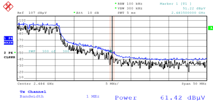
Radiated Restricted Band Edges plot – Peak Reading (802.11g, Ch.11)
