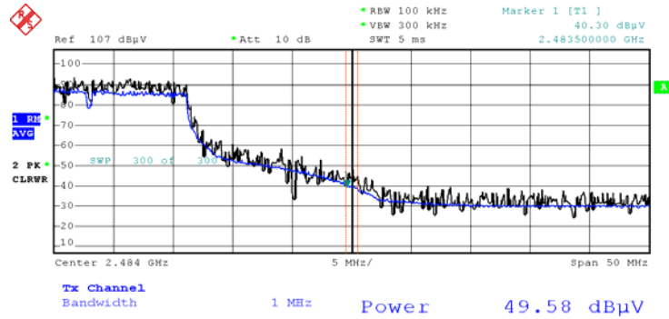
Radiated Restricted Band Edges plot – Average Reading (802.11g, Ch.11)
