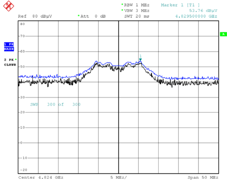
Radiated Spurious Emissions plot – Peak Reading (802.11b_1Mbps, Ch.1 2nd Harmonic)
