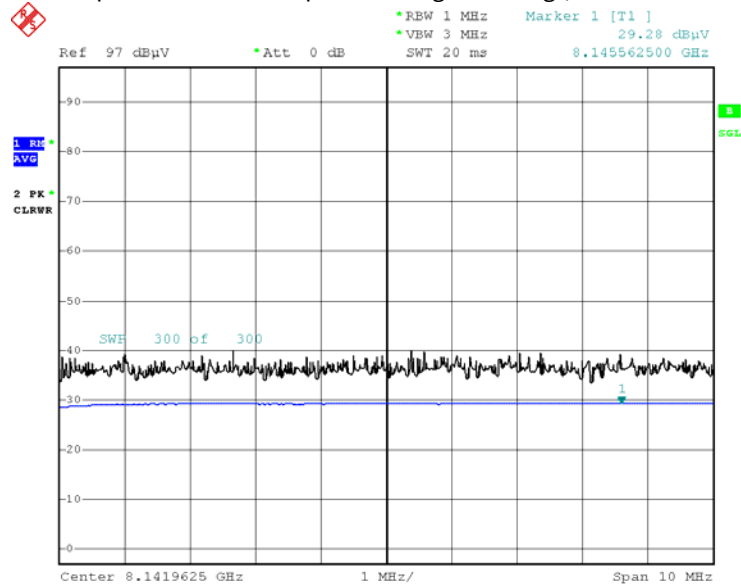
Radiated Spurious Emissions plot – Average Reading (RC2 9th Harmonic)
