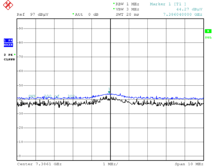
Radiated Spurious Emissions plot – Peak Reading (RC4 8th Harmonic)
