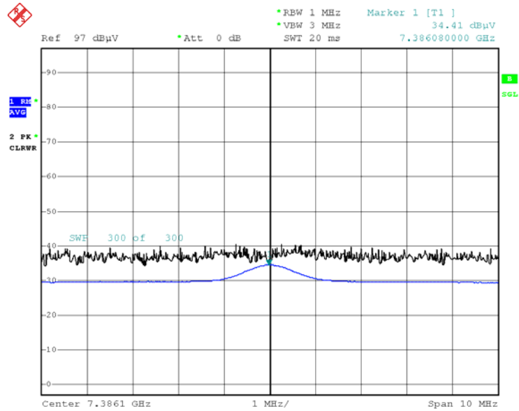
Radiated Spurious Emissions plot –Average Reading (RC4 8th Harmonic)
