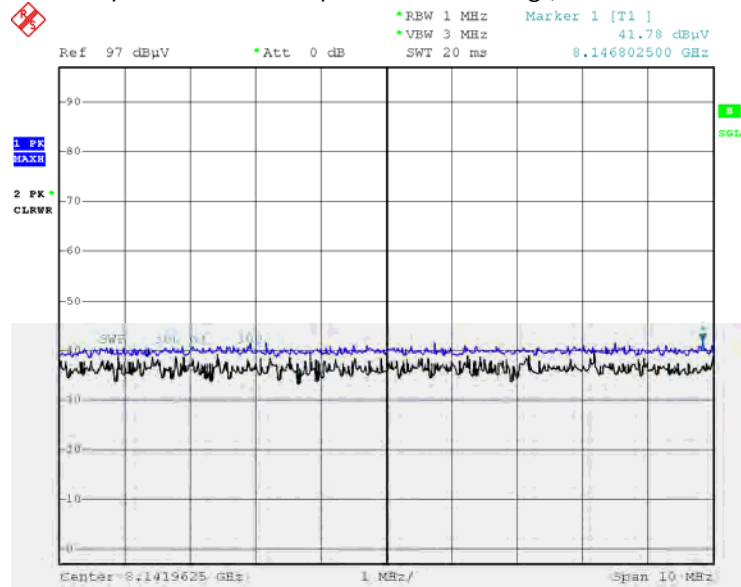
Radiated Spurious Emissions plot – Peak Reading (RC2 9th Harmonic)
