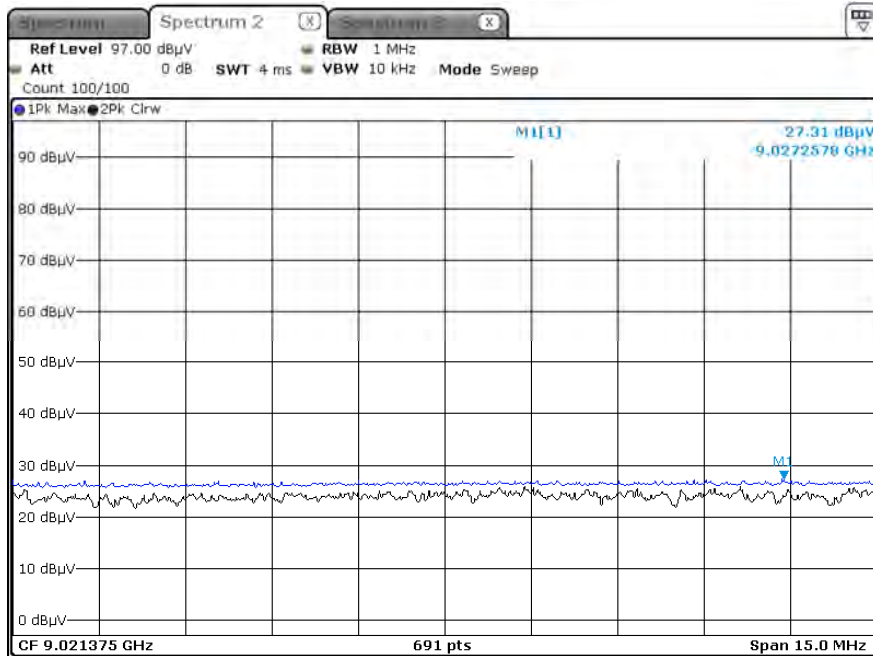
Radiated Spurious Emissions plot – Average Result (RC2 10 th Harmonic)
