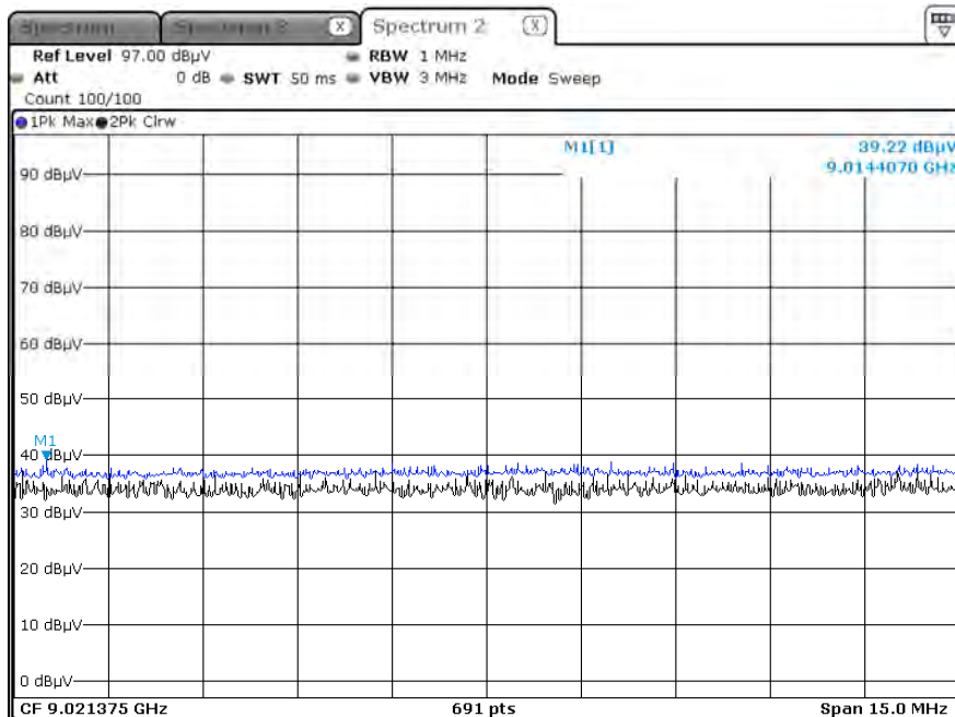
Radiated Spurious Emissions plot – Peak Result (RC2 10 th Harmonic)
