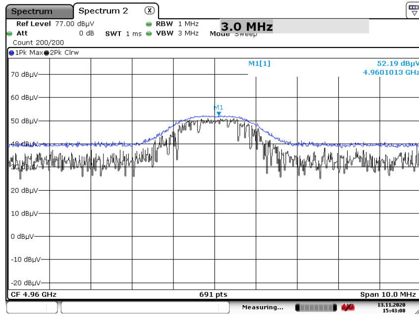
Radiated Spurious Emissions plot – (GFSK, Ch.78 2rd Harmonic, Z-V)
