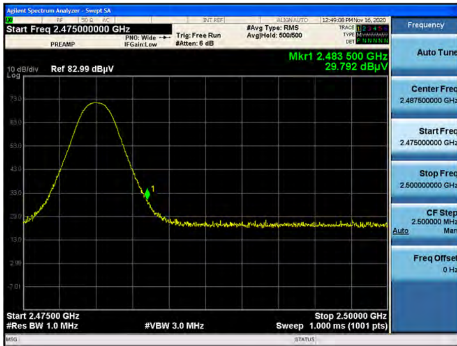
Radiated Restricted Band Edges plot - (8DPSK, Ch.78, X-H)
