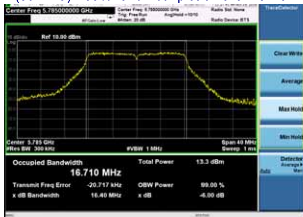
(802.11a) 99%Bandwidth plot on channel 157
