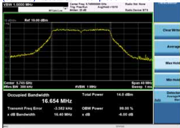
(802.11a) 99%Bandwidth plot on channel 149
