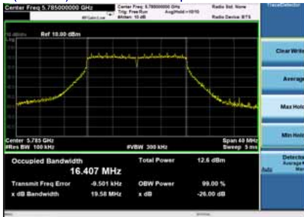
(802.11a) -26dB Bandwidth plot on channel 157
